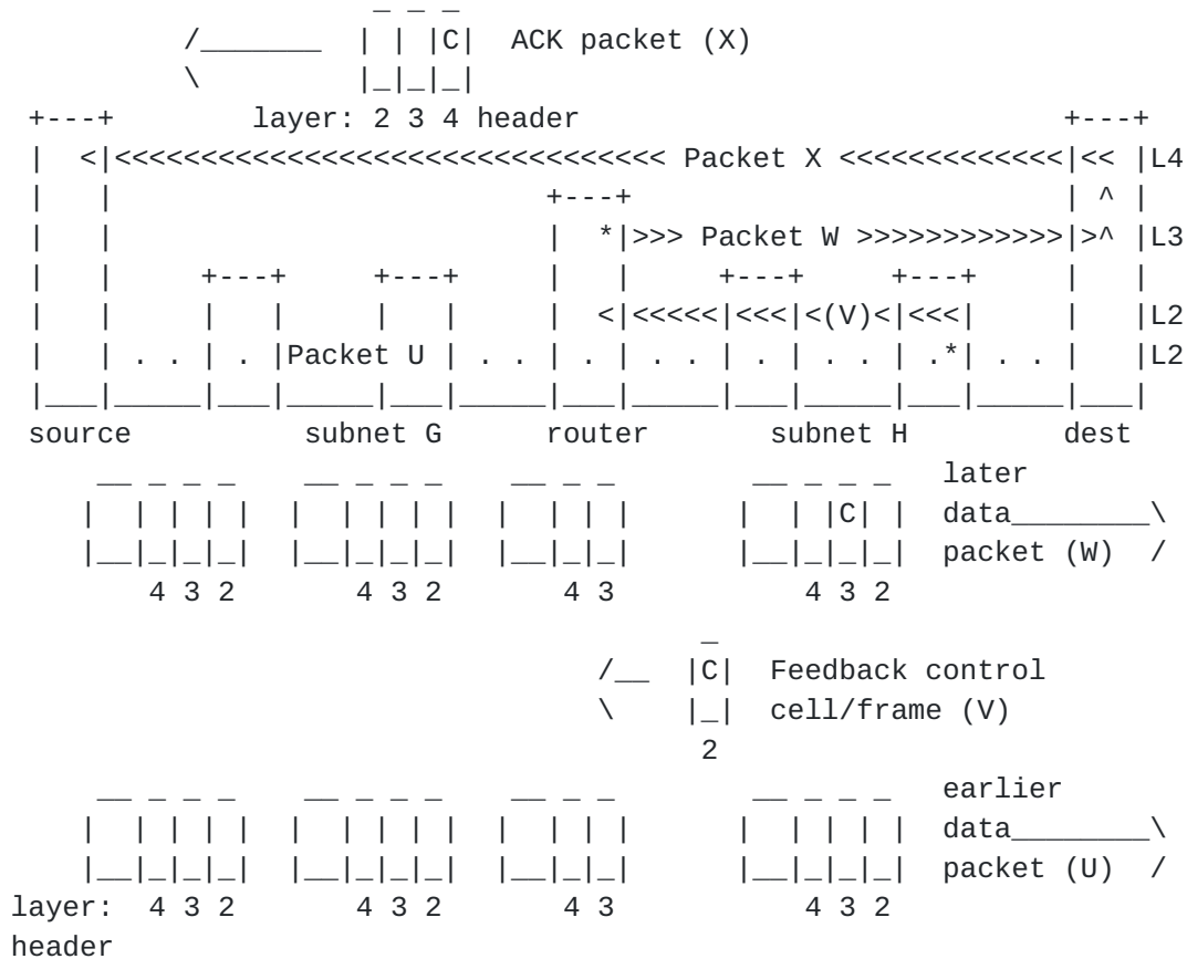
Figure 3: Feed-Backward Mode
