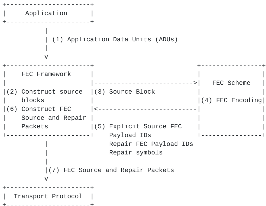
Figure 1: FECFRAME architecture at a sender.
