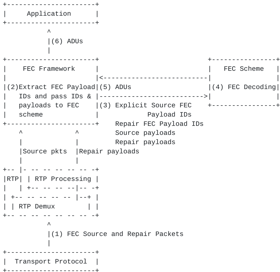
Figure 5: Receiver Operation with Sliding Window FEC Codes and RTP Repair Flows
