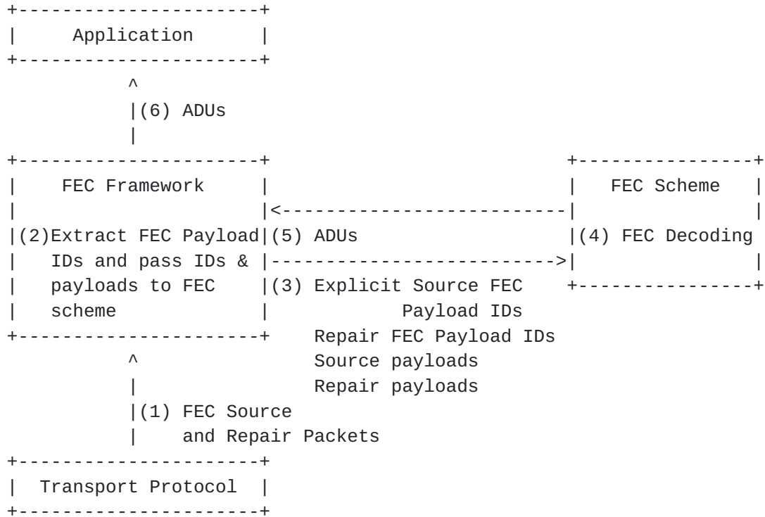
Figure 4: Receiver Operation with Sliding Window FEC Codes
