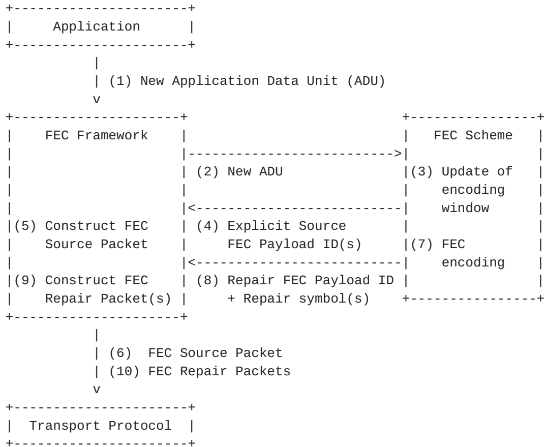
Figure 2: Sender Operation with Sliding Window FEC Codes
