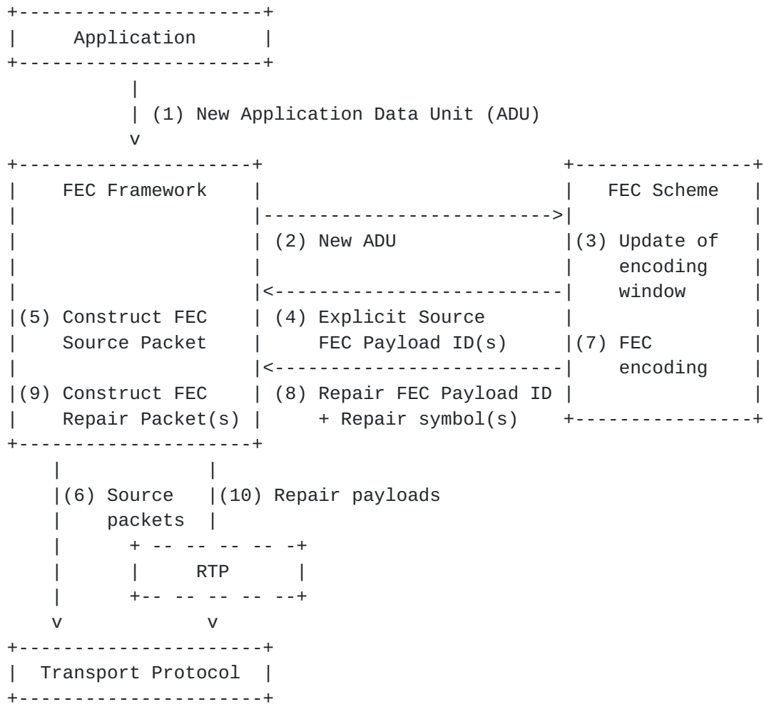
Figure 3: Sender Operation with Sliding Window FEC Codes and RTP Repair Flows
