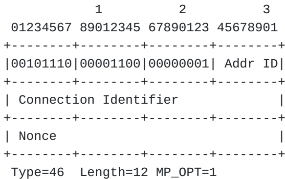
Figure 9: Format of the MP_JOIN suboption
