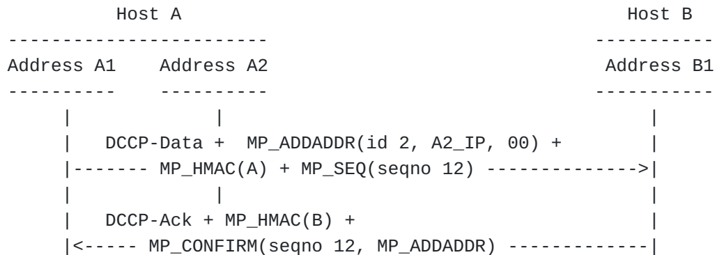
Figure 22: Example MP-DCCP ADDADDR procedure
