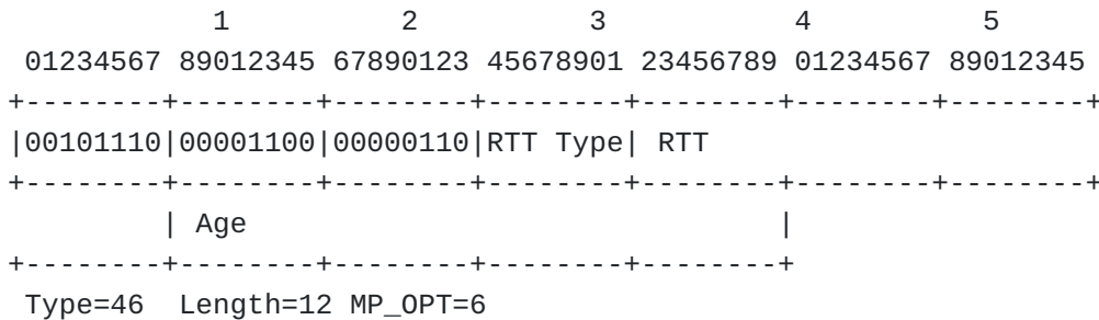
Figure 14: Format of the MP_RTT suboption
