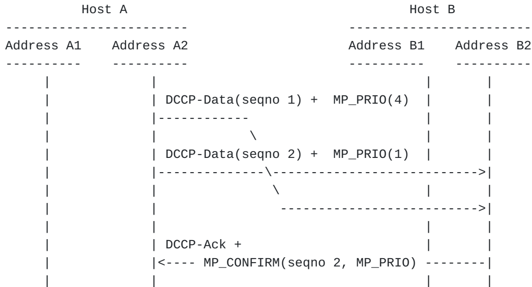
Figure 8: Example MP-DCCP CONFIRM procedure with outdated suboption
