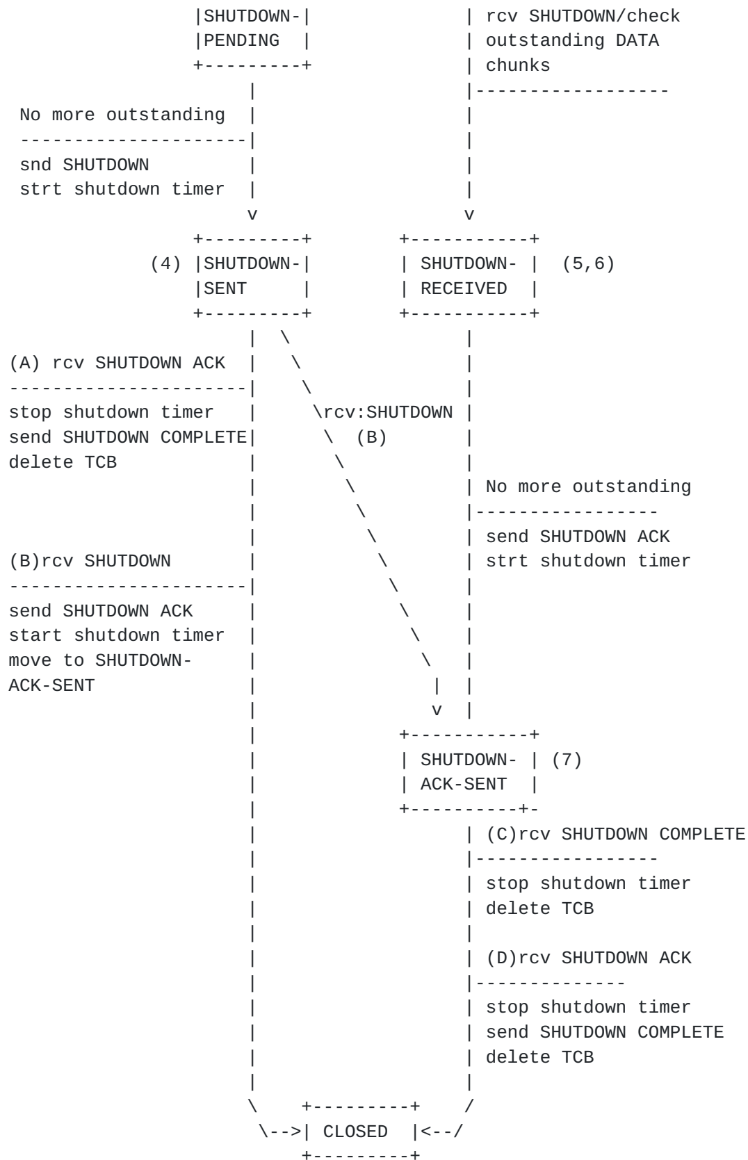
Figure 3: State Transition Diagram of SCTP
