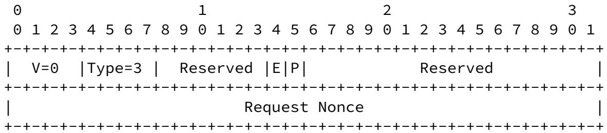
Figure 2: Updated AMT Request Message Format
