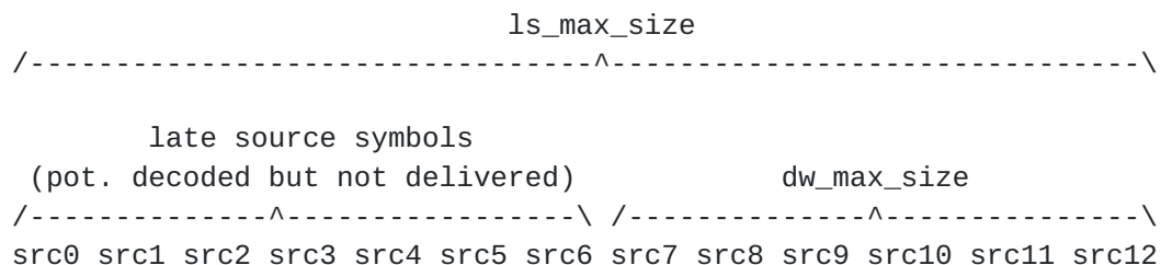
Figure 13: Relationship between parameters to decode beyond maximum latency.
