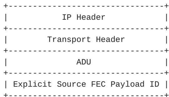
Figure 5: Structure of an FEC Source Packet with the Explicit Source FEC Payload ID
