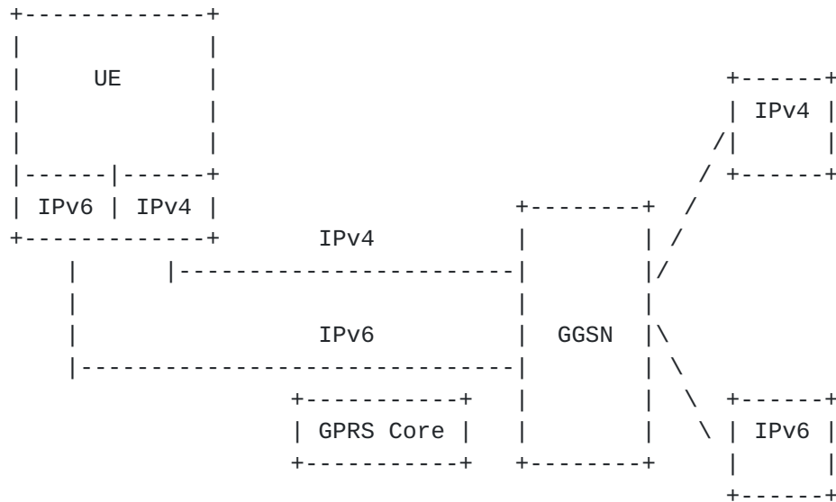
Figure 3: Dual-Stack Case
