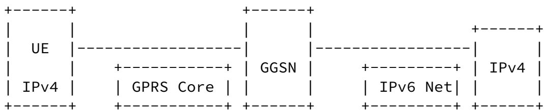
Figure 5: IPv4 nodes communicating over IPv6
