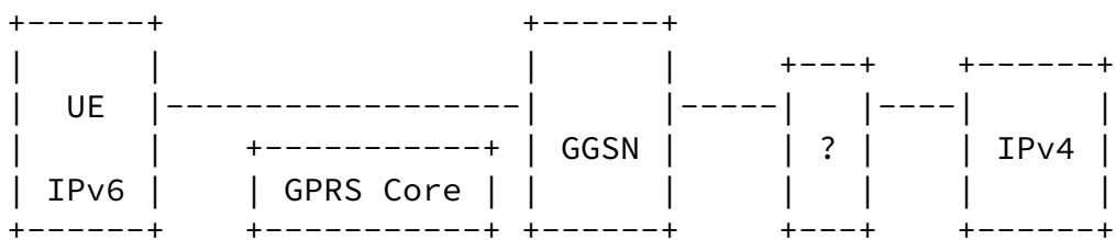
Figure 6: IPv6 node communicating with IPv4 node
