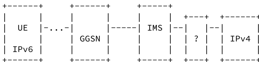
Figure 8: IMS UE connecting to an IPv4 node
