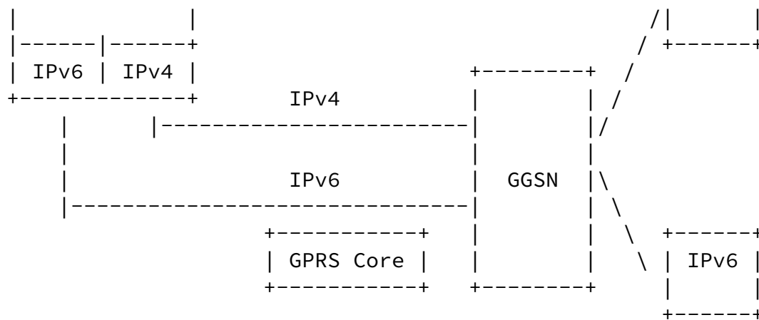
Figure 3: Dual-Stack Case
