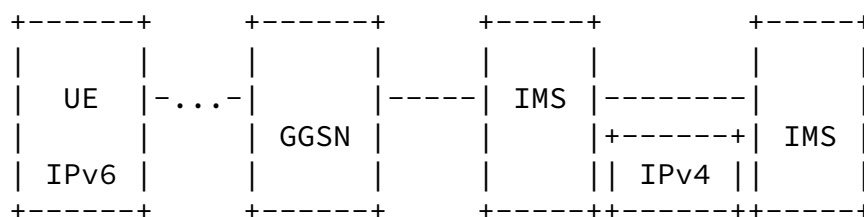
Figure 9: Two IMS islands connected over IPv4
