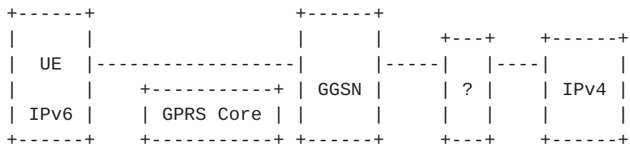
Figure 6: IPv6 node communicating with IPv4 node
