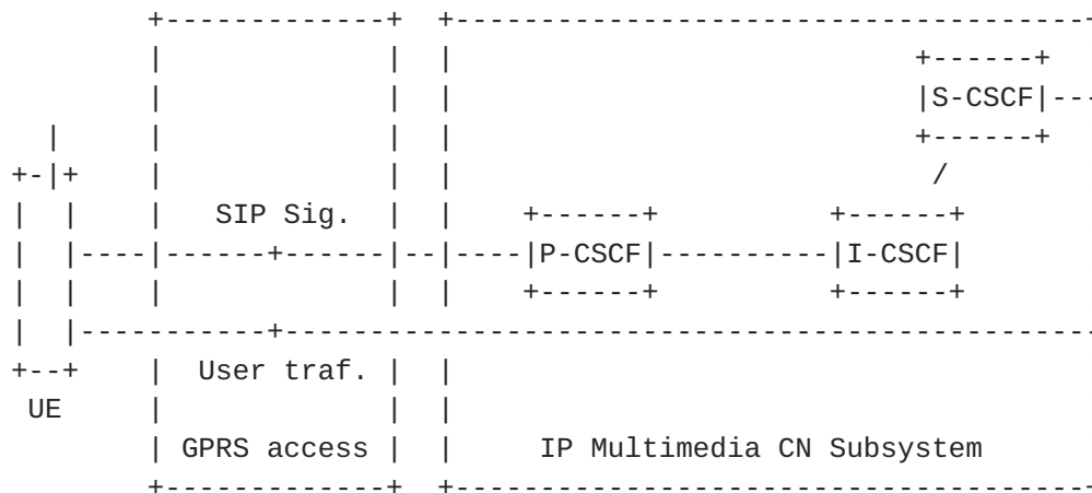
Figure 2: Overview of the 3GPP IMS architecture
