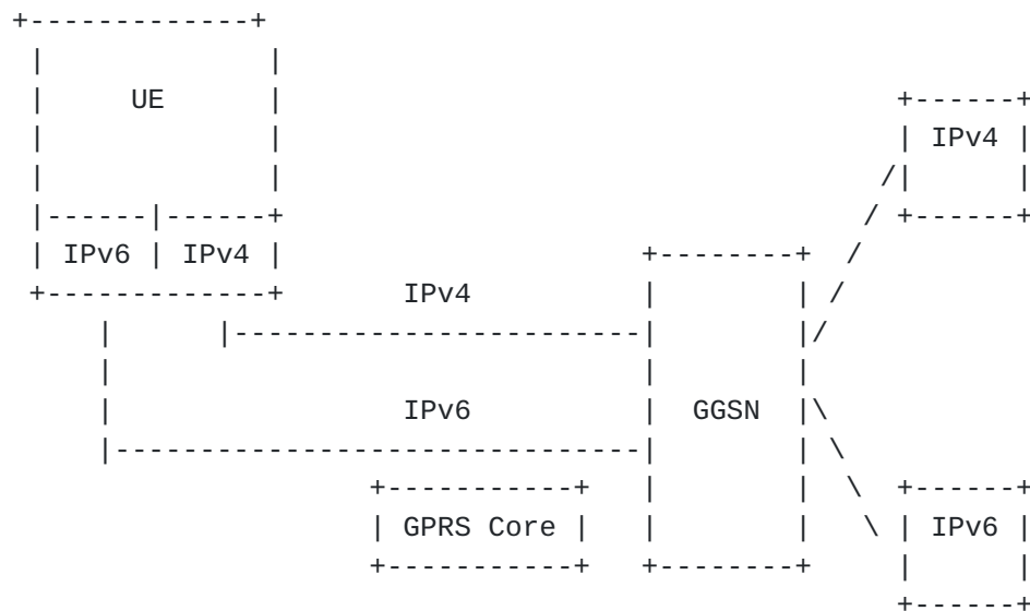
Figure 3: Dual-Stack Case
