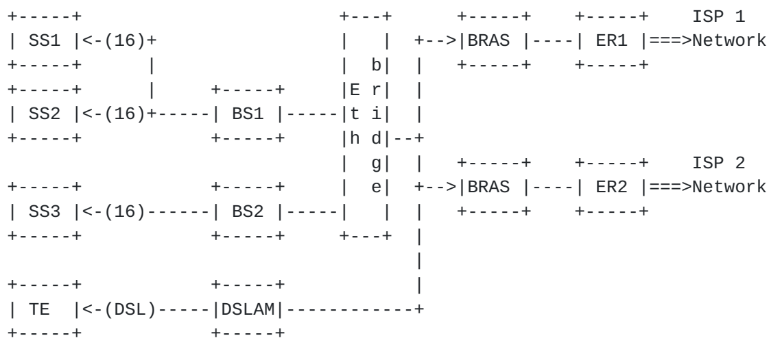
Figure 5: Integration of 802.16 access into DSL infrastructure
