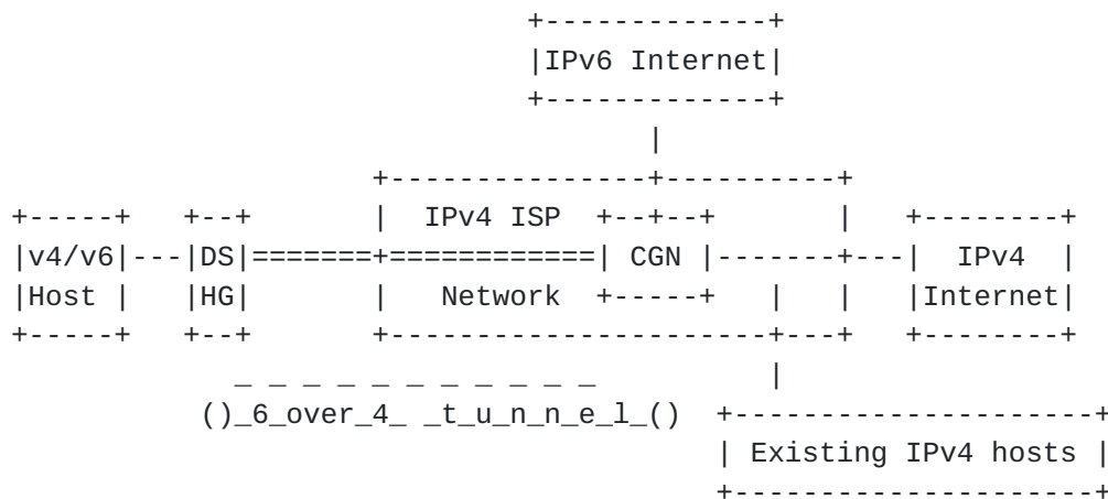
Figure 1: incremental CGN approach with IPv4 ISP network
