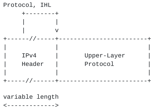
Figure 1: IPv4 Packet Structure
