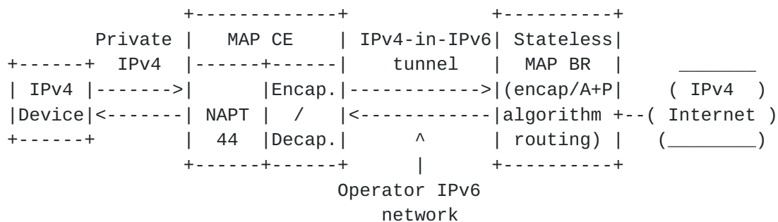
Figure 4: Overview of the MAP-E architecture
