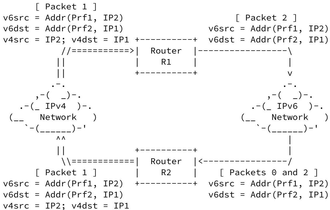
Figure 1: The network setting of the attack
