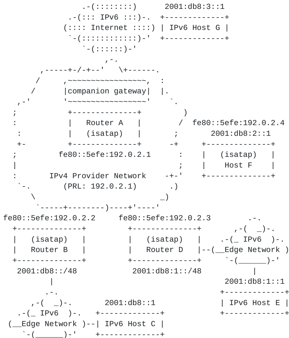
Figure 3: Reference ISATAP Network Topology
