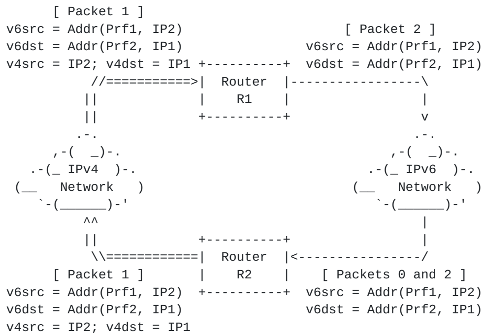
Figure 1: The network setting of the attack
