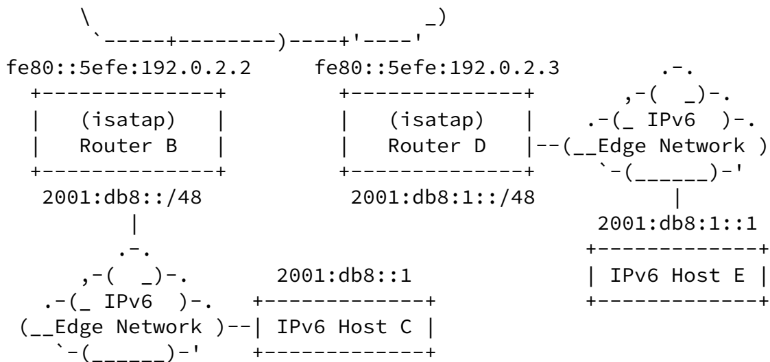
Figure 3: Reference ISATAP Network Topology
