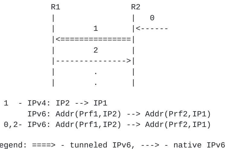
Figure 2: Routing loop attack between two tunnels' routers
