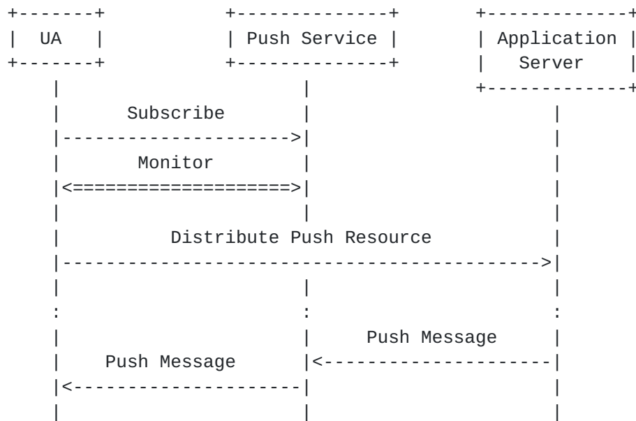
Figure 1: Webpush Architecture
