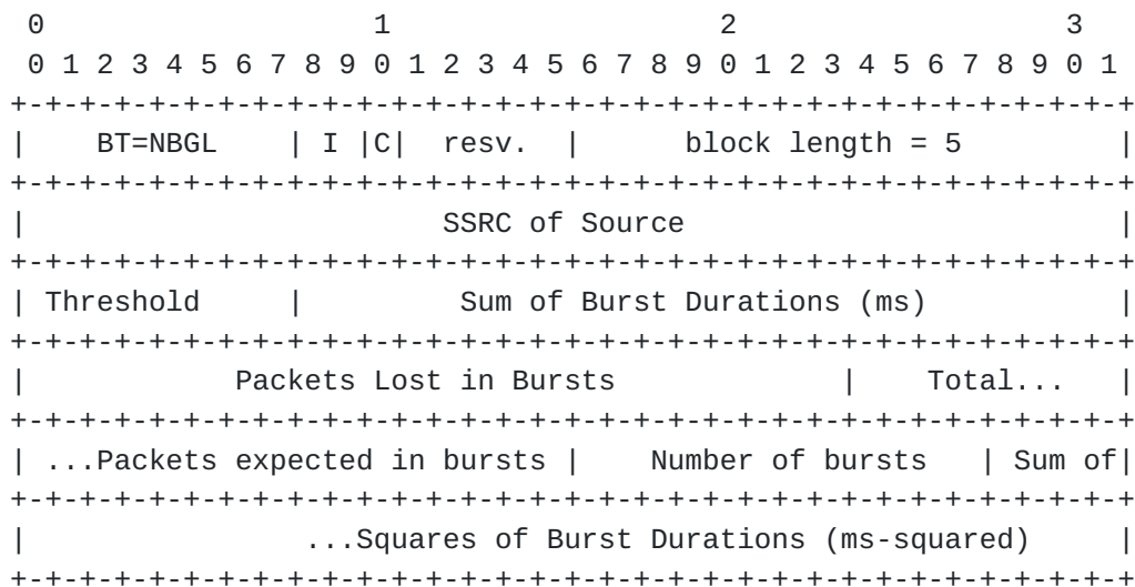
Figure 1: Report Block Structure
