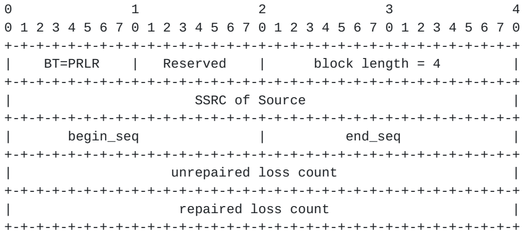
Figure 1: Format for the Post-Repair Loss Count Metrics Report Block
