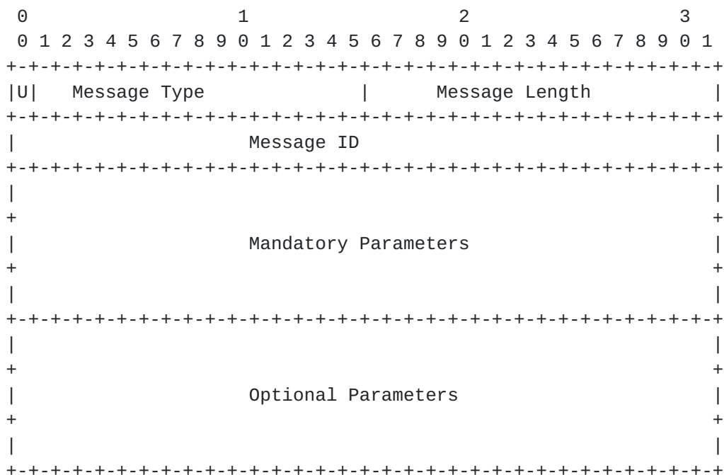
Figure 17: LDP message format
