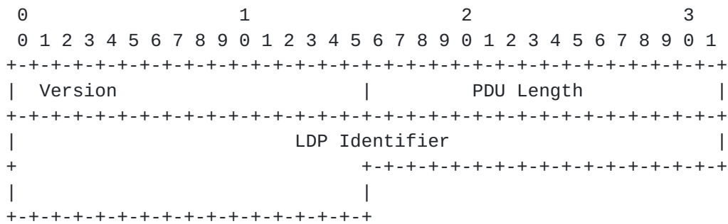
Figure 2: LDP PDU
