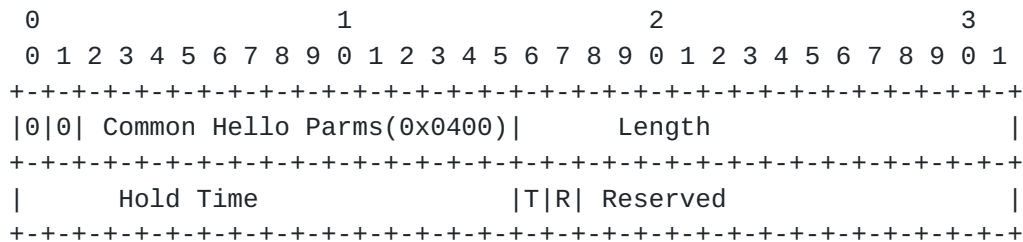
Figure 20: Hello Message
