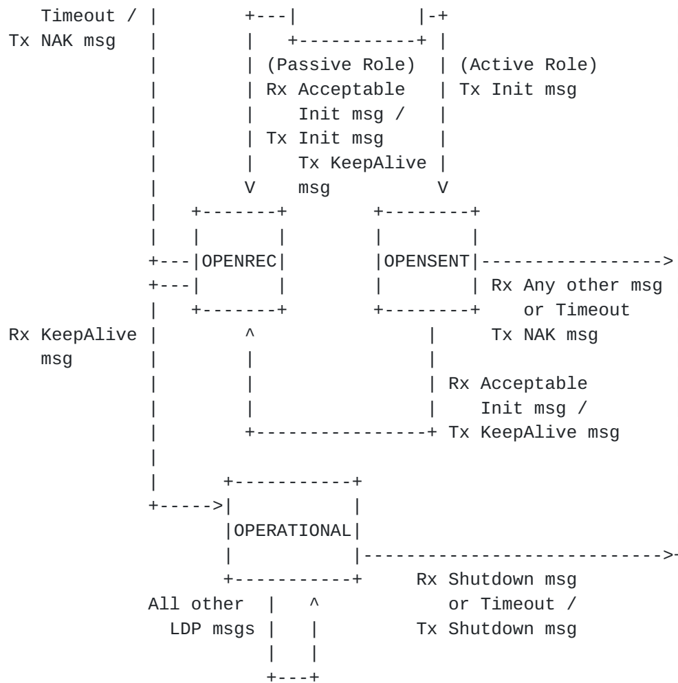
Figure 1: LDP State Machine
