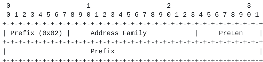
Figure 5: Prefix FEC Element Value Encoding
