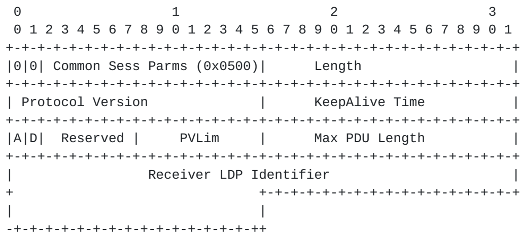
Figure 22: Common Session Parameters TLV
