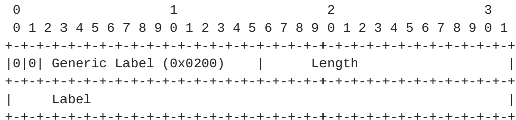
Figure 6: Generic Label
