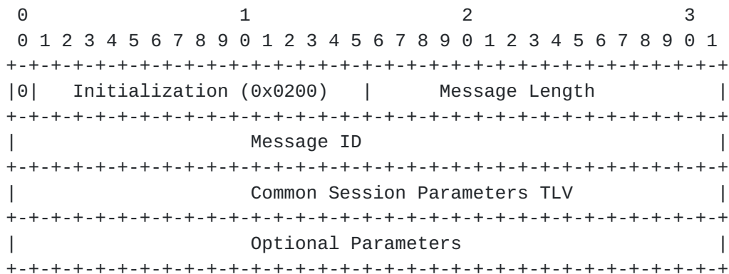
Figure 21: Initialization Message
