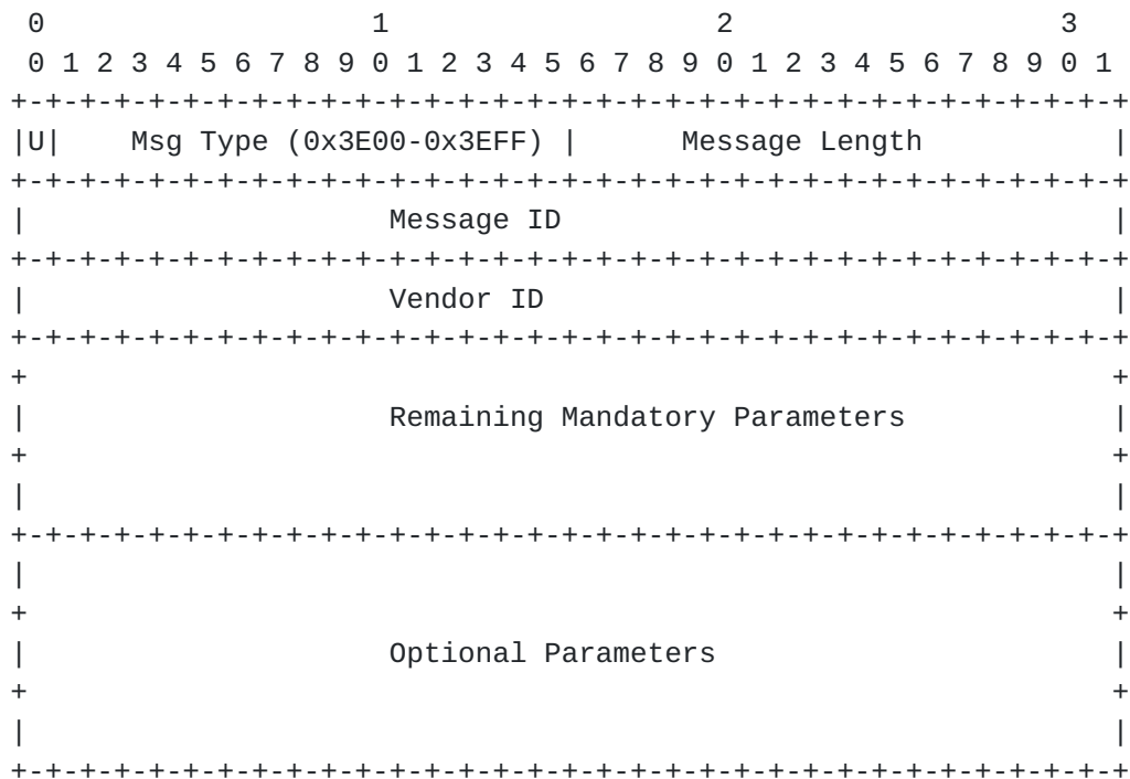
Figure 36: LDP Vendor-Private Messages
