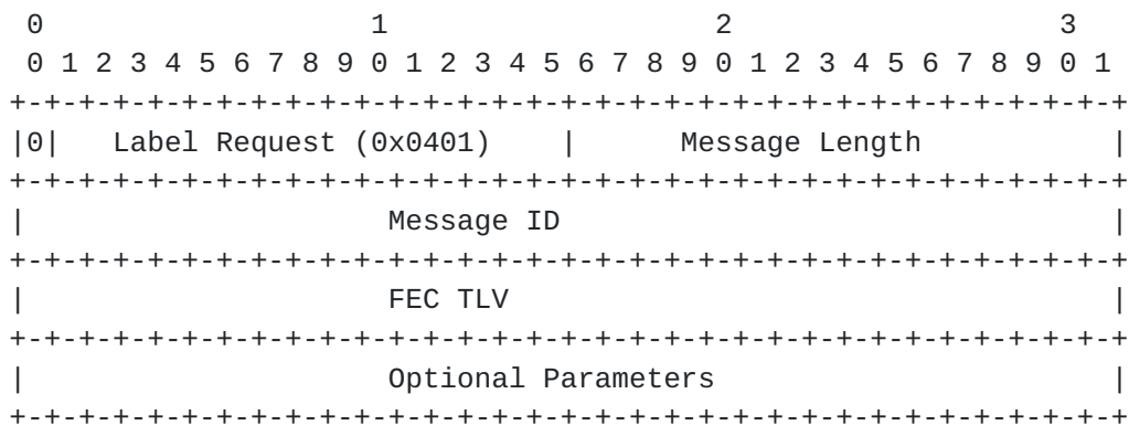
Figure 31: Label Request Message
