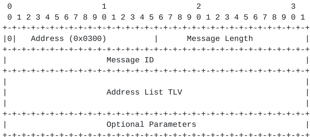
Figure 28: Address Message
