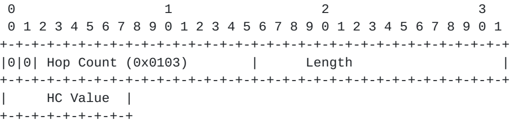
Figure 13: Hop Count TLV
