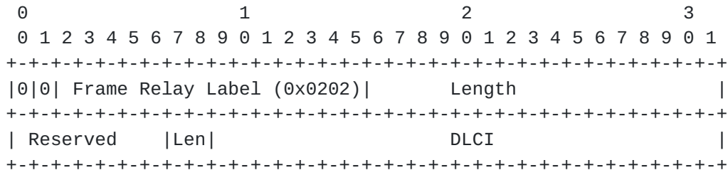
Figure 9: Frame Relay Label TLV
