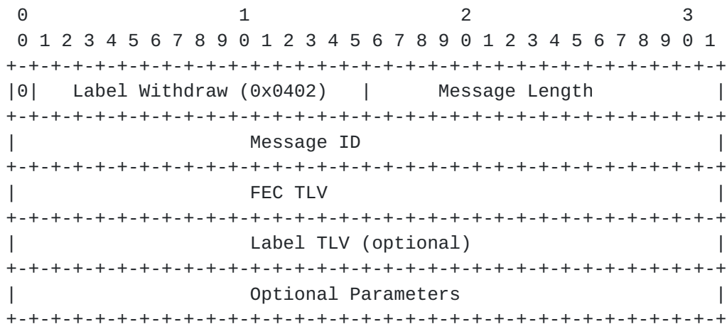
Figure 33: Label Withdraw Message
