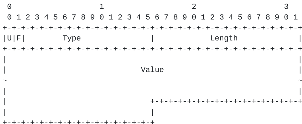
Figure 3: TLV Encoding
