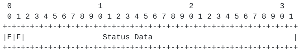
Figure 16: Path Vector TLV
