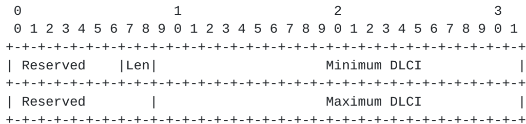
Figure 26: Frame Relay Label Range Component
