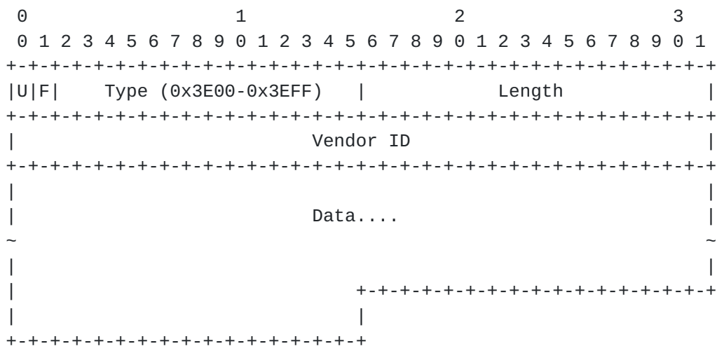
Figure 35: LDP Vendor-Private TLVs
