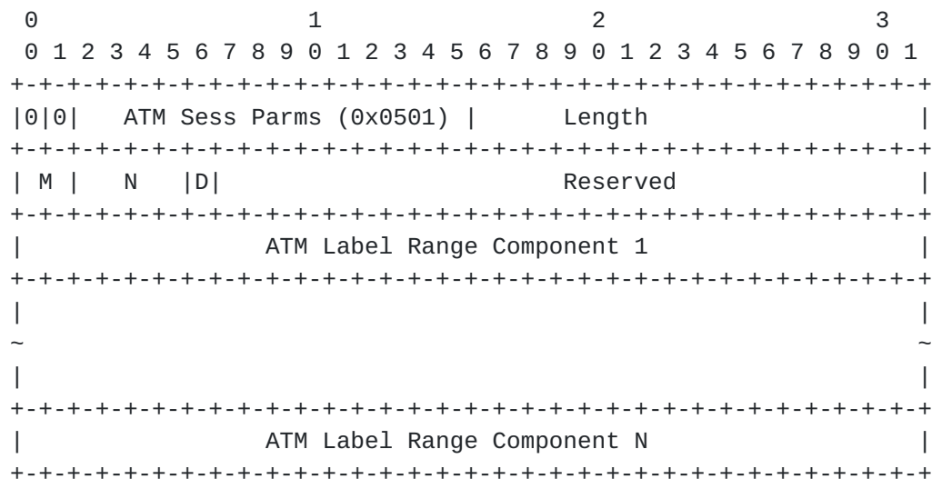
Figure 23: ATM Session Parameters (optional)
