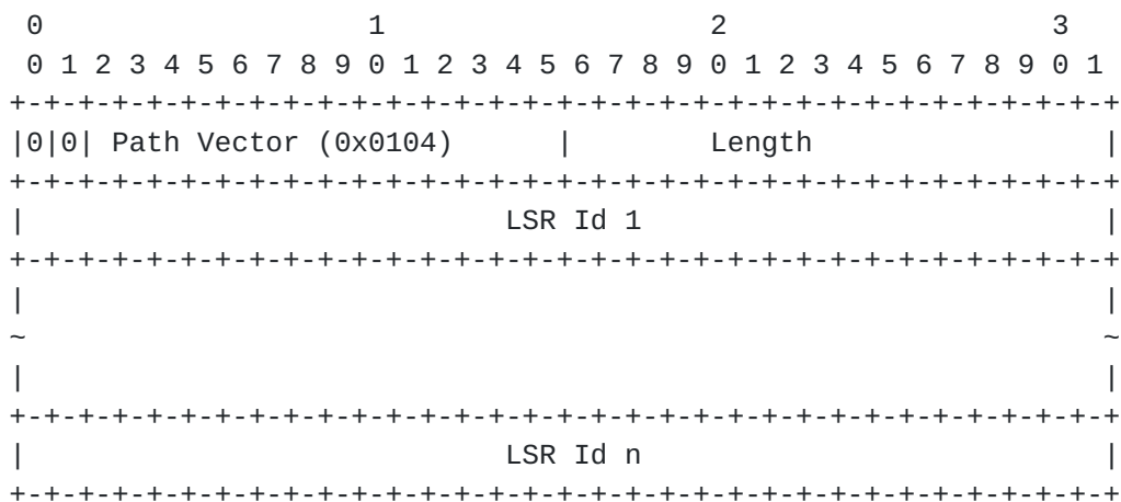
Figure 14: Path Vector TLV
