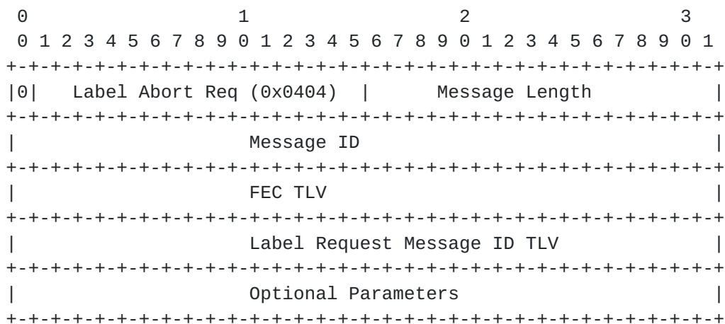
Figure 32: Label Abort Request Message
