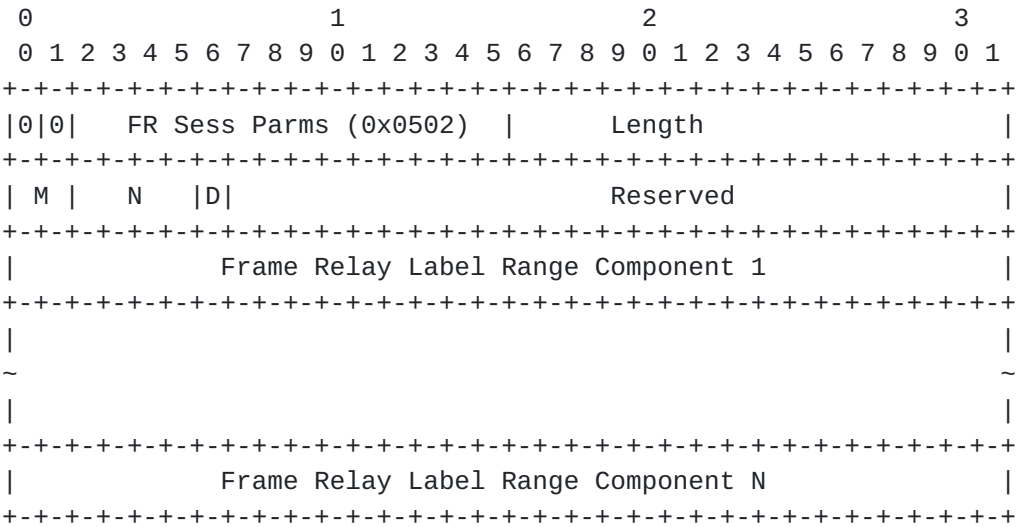
Figure 25: Frame Relay Session Parameters
