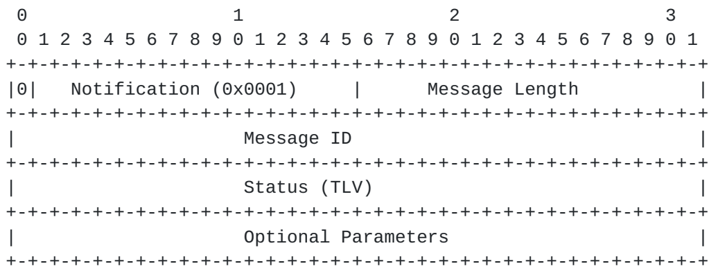
Figure 18: Notification Message
