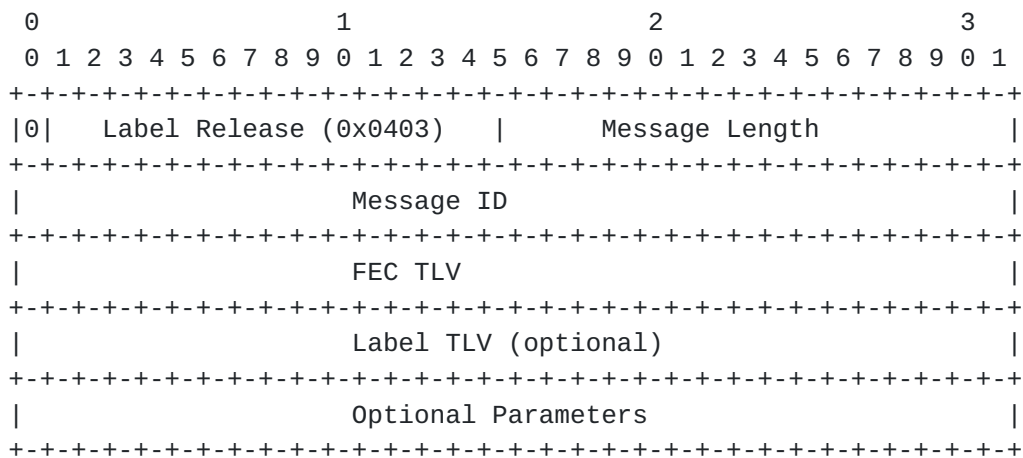
Figure 34: Label Release Message
