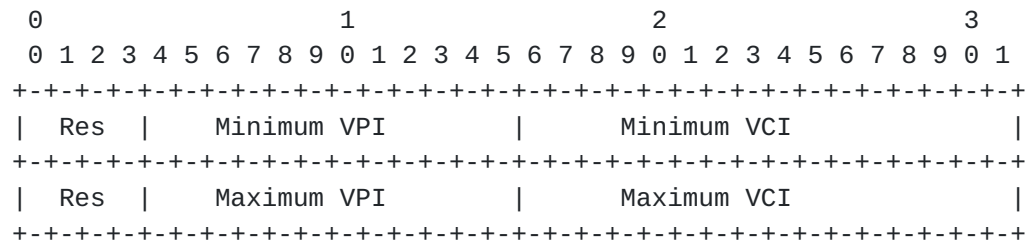
Figure 24: ATM Label Range Component
