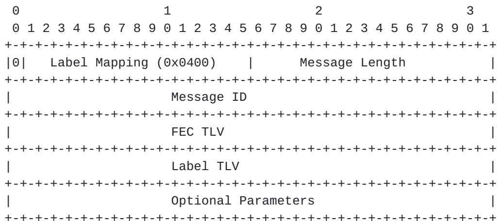
Figure 30: Label Mapping Message
