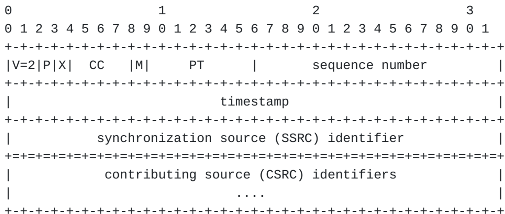
Figure 1: RTP Header
