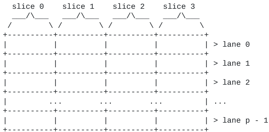
Single-pass Argon2 with p lanes and 4 slices
