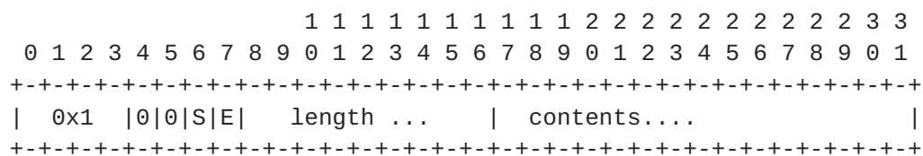
Figure 4: Format of bundle data segment messages
