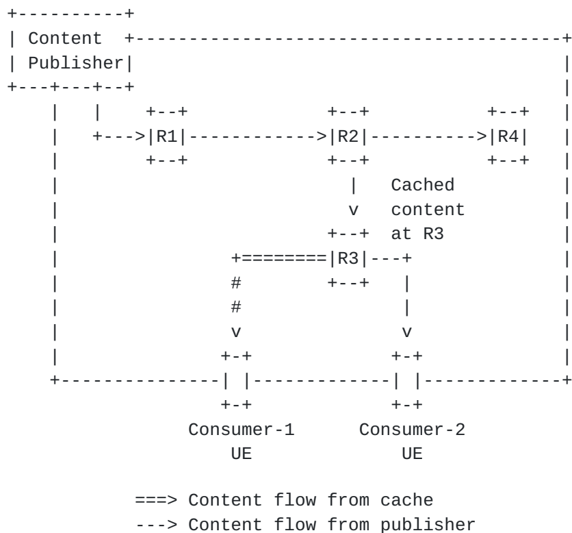
Fig. 2. ICN Architecture
