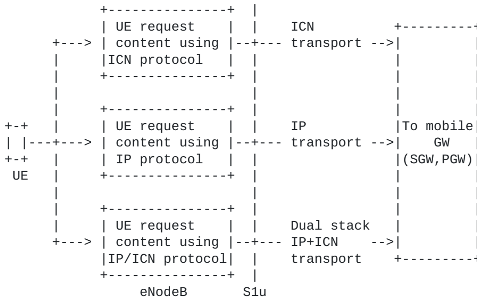
Figure 8: Native ICN Deployment in eNodeB
