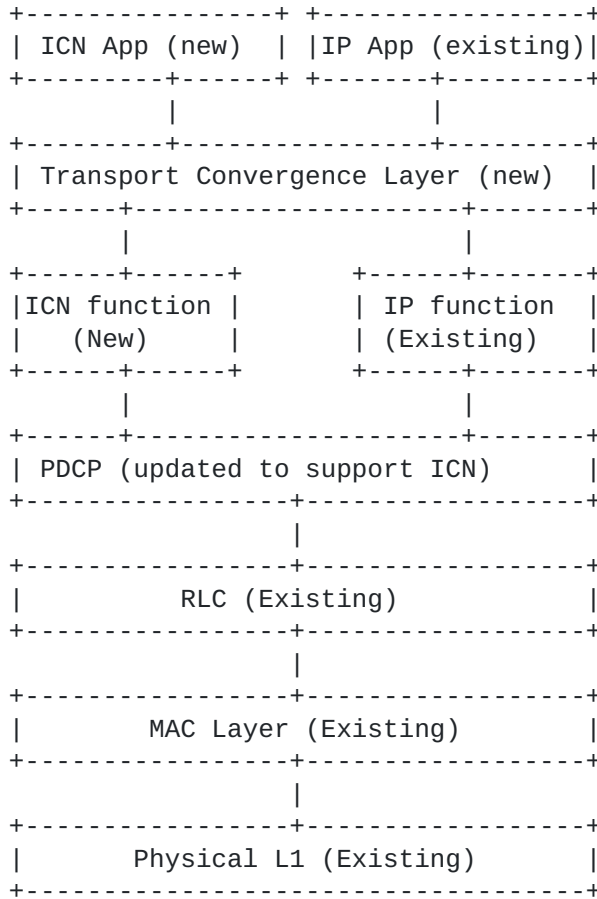
Figure 6: Dual stack ICN protocol interactions
