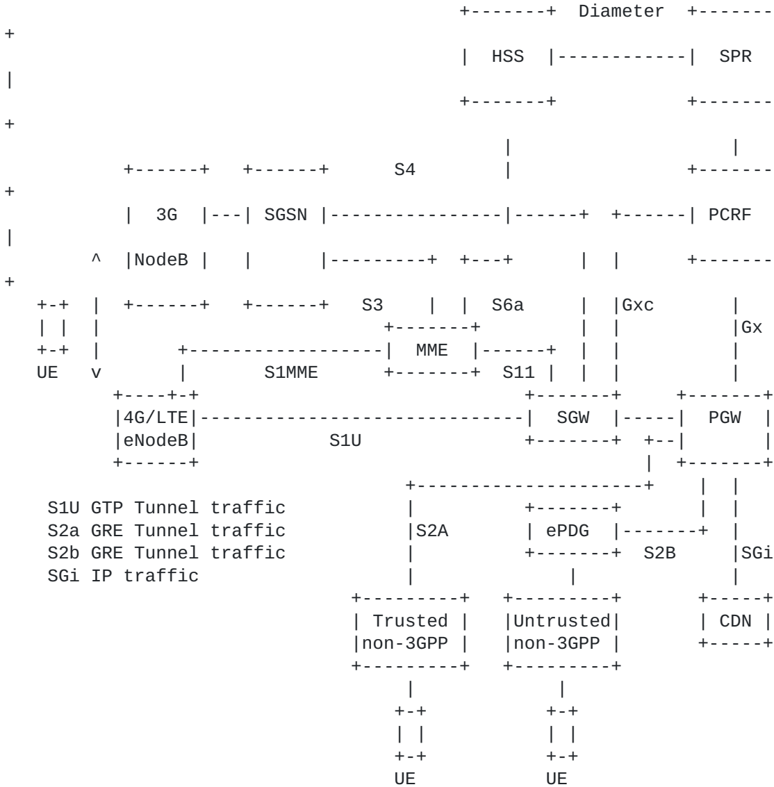
Figure 1: LTE, 4G Mobile Network Overview
