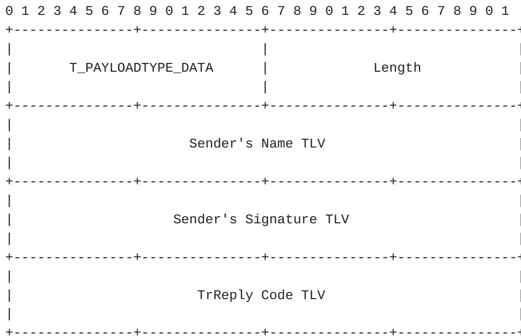
Figure 6: Traceroute Reply Message Format
