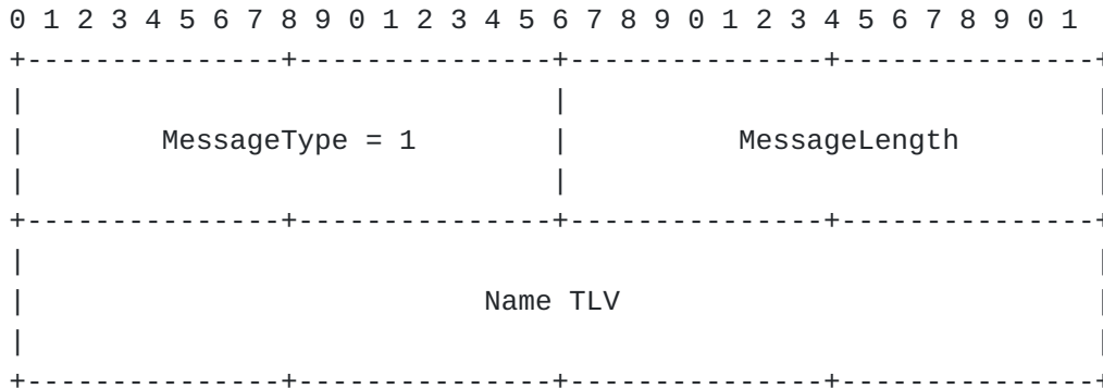
Figure 2: Traceroute Request Message Format
