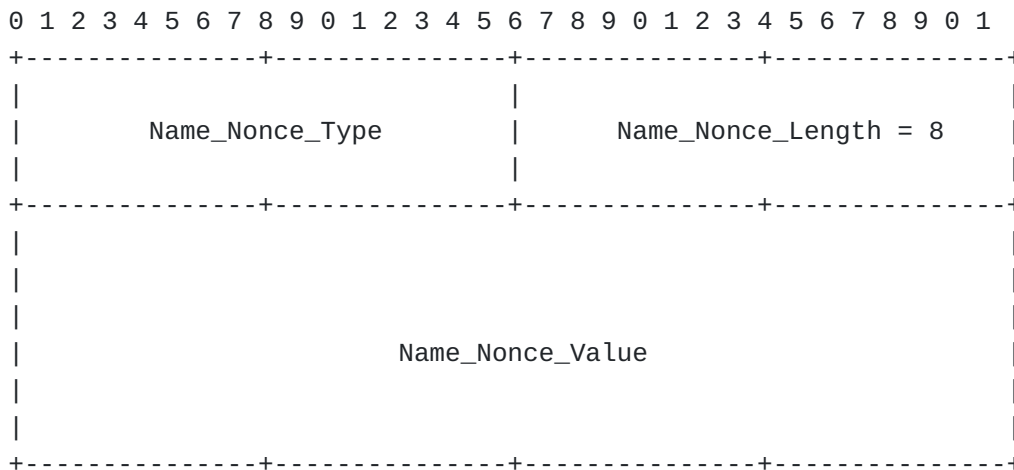
Figure 3: Name Nonce Typed Component TLV
