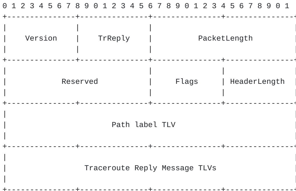
Figure 4: Traceroute Reply CCNx Packet Format
