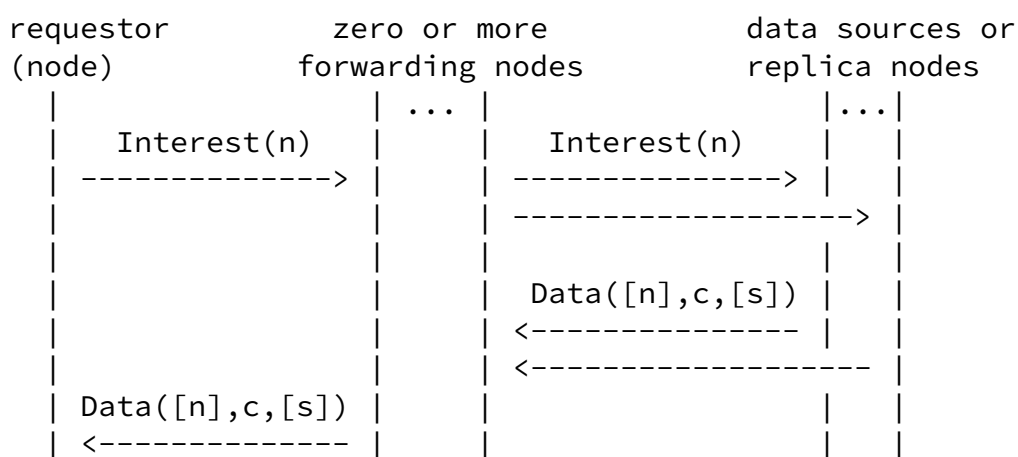
Figure 1: Request-Reply Protocol of ICN networking. Legend: n=name, c=content, s=signature.
