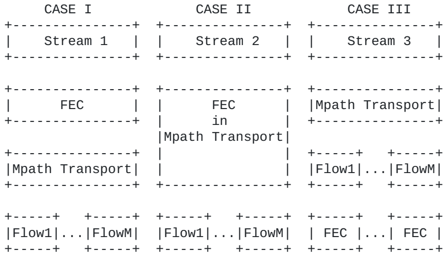
Figure 5: Transport multipath and single stream applications - in the scope of the document
