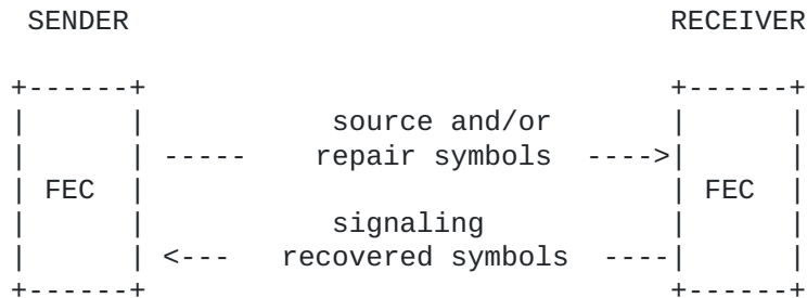
Figure 2: Forward Erasure Correction (FEC) channel
