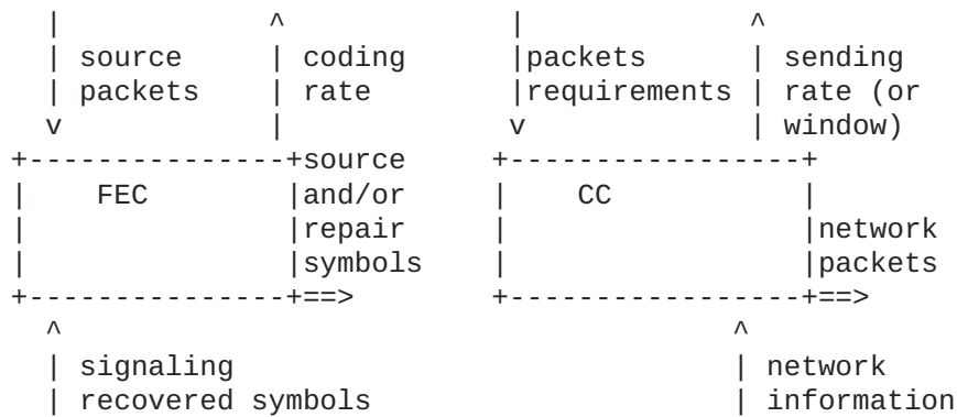
Figure 3: Separate entities (sender-side)
