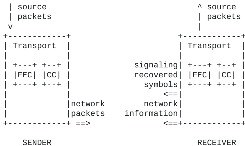
Figure 8: FEC in the transport
