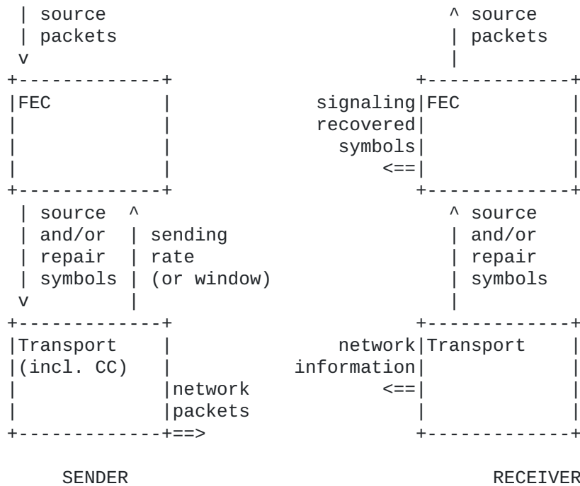
Figure 7: FEC above the transport
