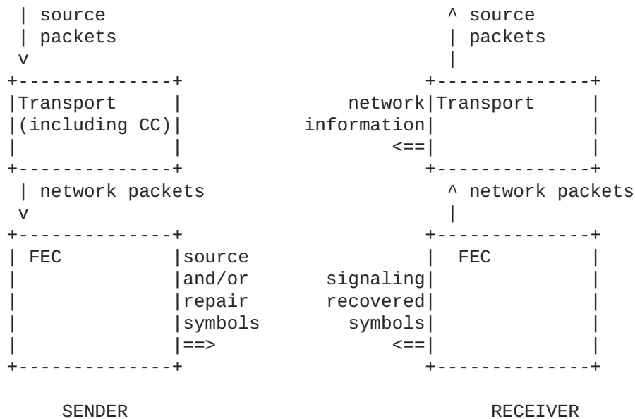
Figure 9: FEC below the transport
