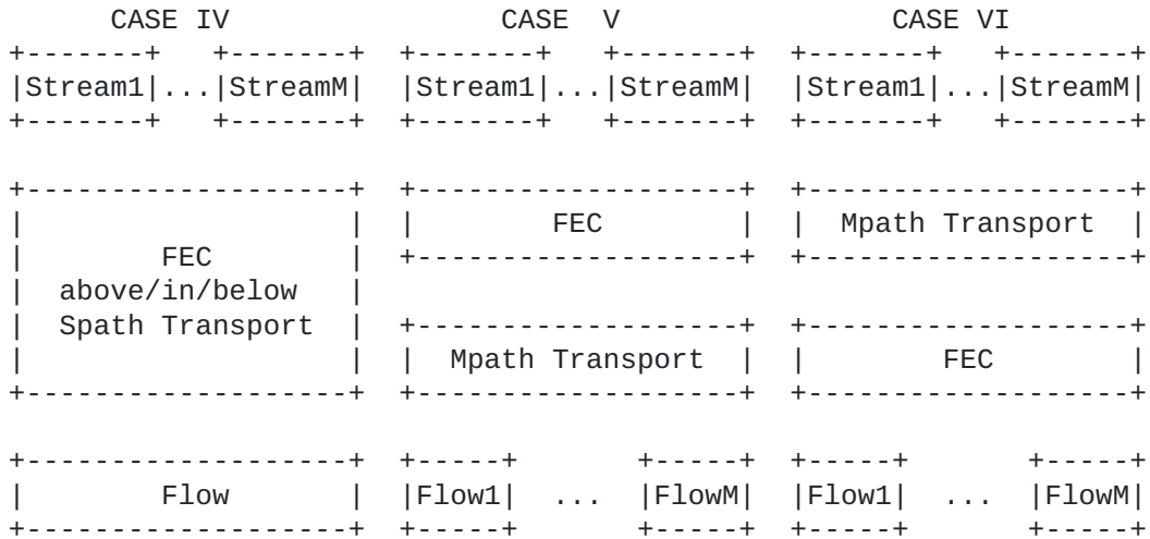
Figure 6: Transport single path, transport multipath and multi-stream applications - out of the scope of the document
