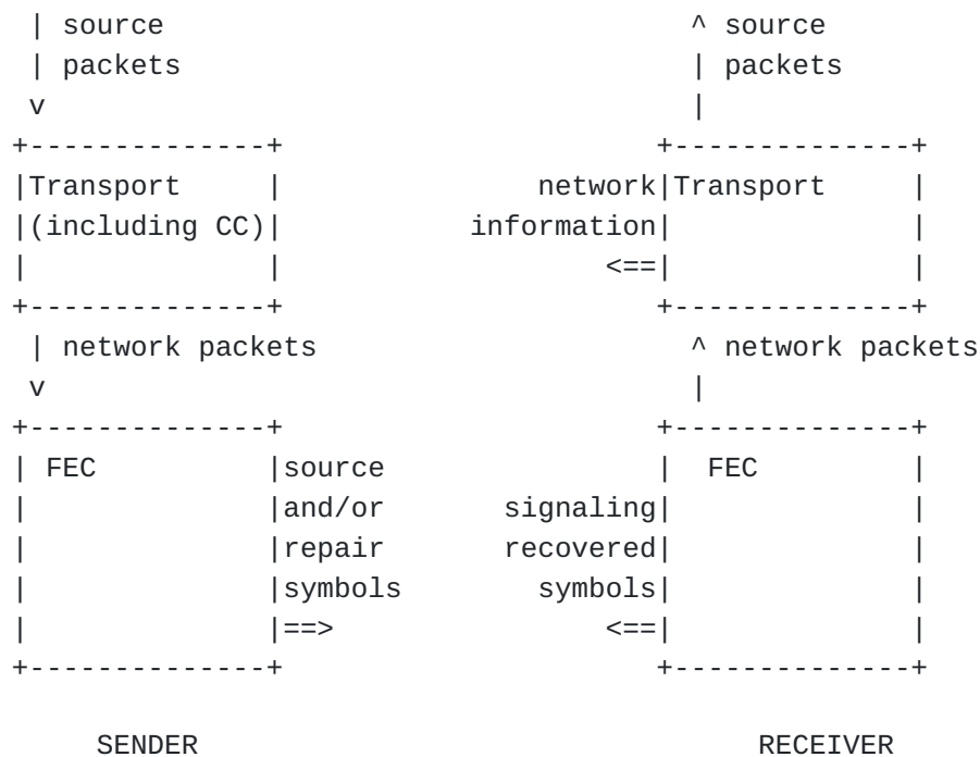
Figure 9: FEC below the transport
