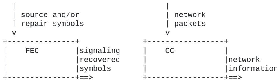
Figure 4: Separate entities (receiver-side)
