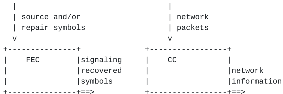
Figure 3: Separate entities (sender-side)
