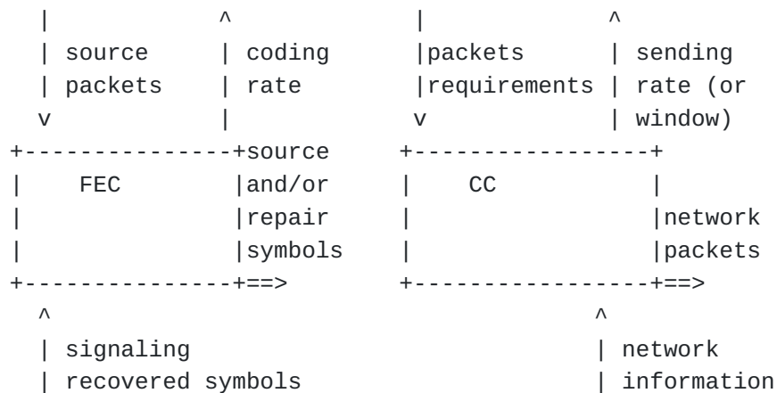
Figure 3: Separate entities (sender-side)
