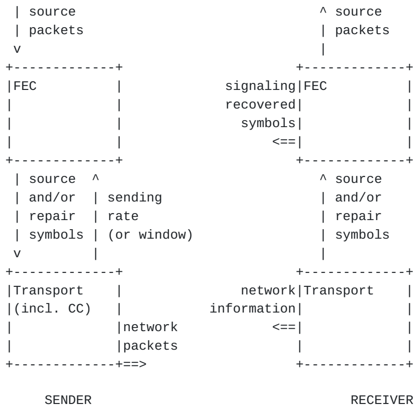
Figure 7: FEC above the transport
