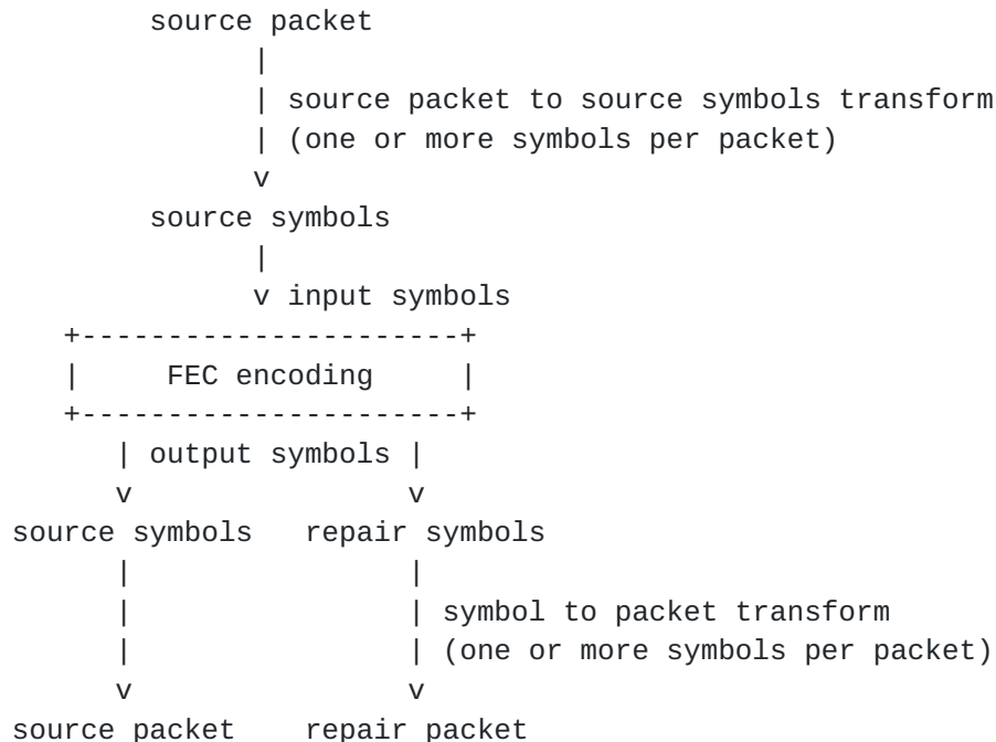
Figure 1: Packet and symbol relationships at a Coding Node that performs Encoding (rather than Recoding).
