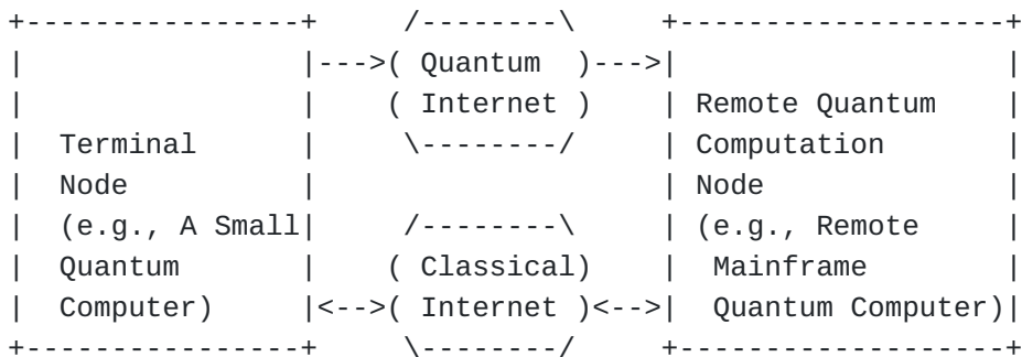
Figure 2: Secure Quantum Computing with Privacy Preservation
