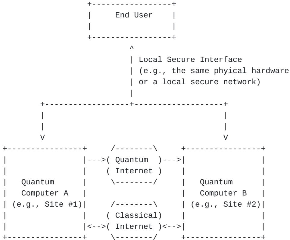
Figure 3: Distributed Quantum Computing
