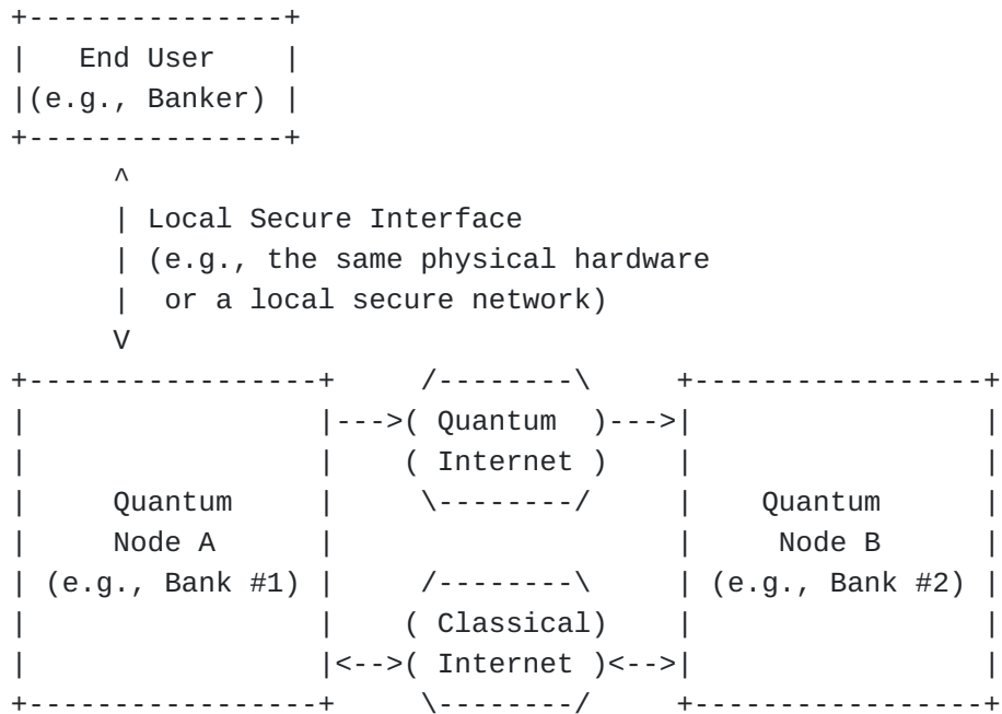
Figure 1: Secure Communication Setup
