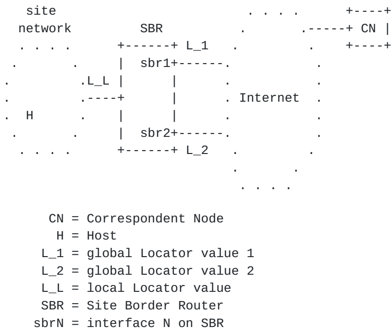
Figure 3.1: Alternative site multi-homing example with an SBR.
