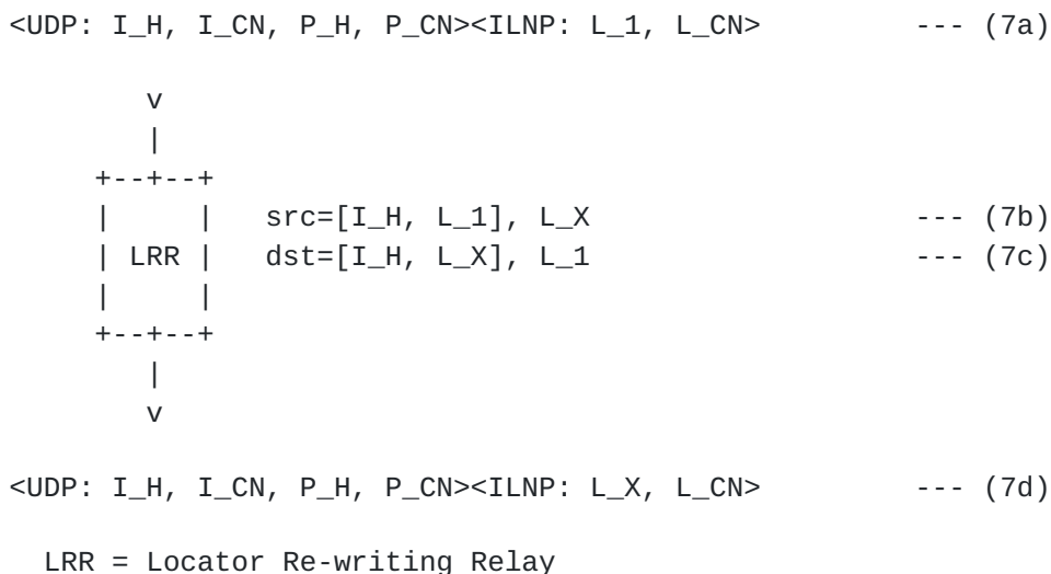
Figure 7.1: Locator Re-Writing Relay (LRR) example
