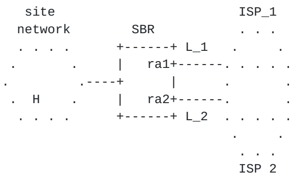
Figure 6.2b: ILNP mobile network during handover.
