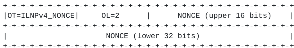
Figure 3: ILNP Nonce Option for IPv4
