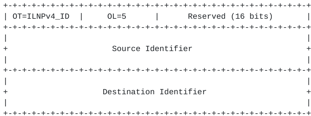
Figure 2: ILNP Identifier Option for IPv4
