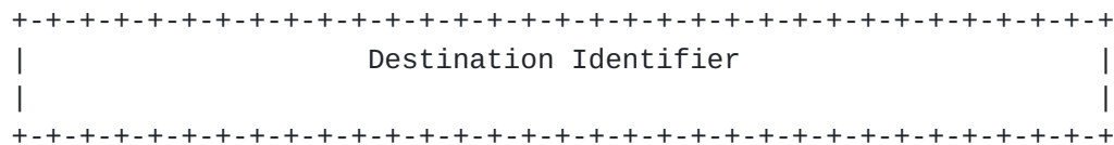
Figure 2: ILNP Identifier Option for IPv4
