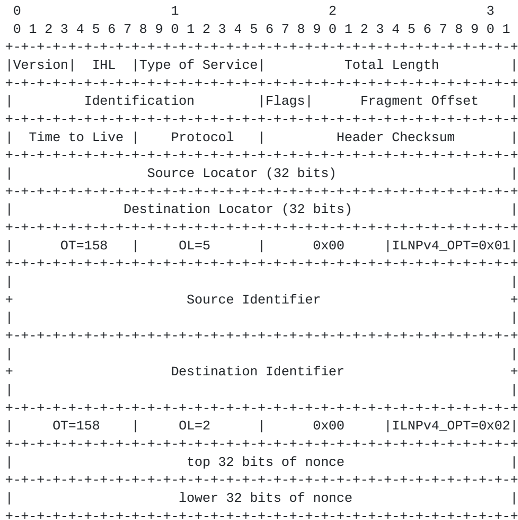
Figure 1: ILNPv4 header with ILNP ID option and ILNP Nonce option.
