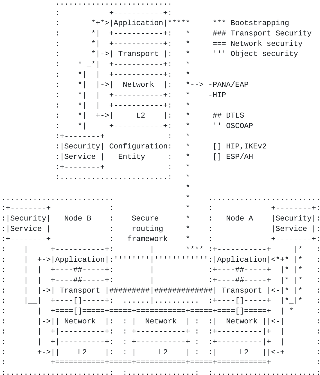
Figure 4: Relationships between IP-based security protocols
