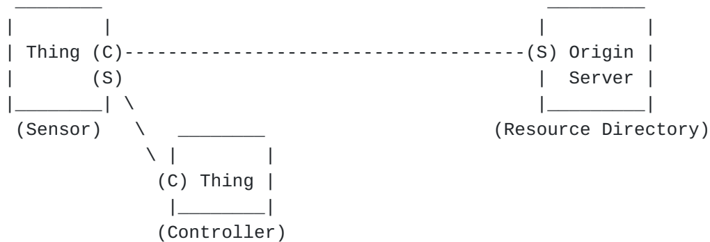
Figure 4: Constrained RESTful environments
