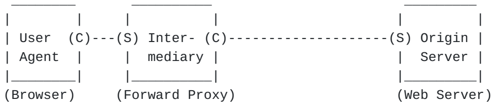
Figure 2: Communication with Forward Proxy
