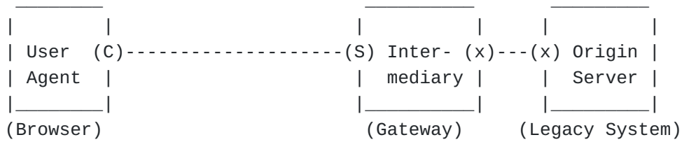
Figure 3: Communication with Reverse Proxy
