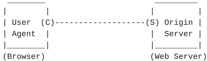
Figure 1: Client-Server Communication
