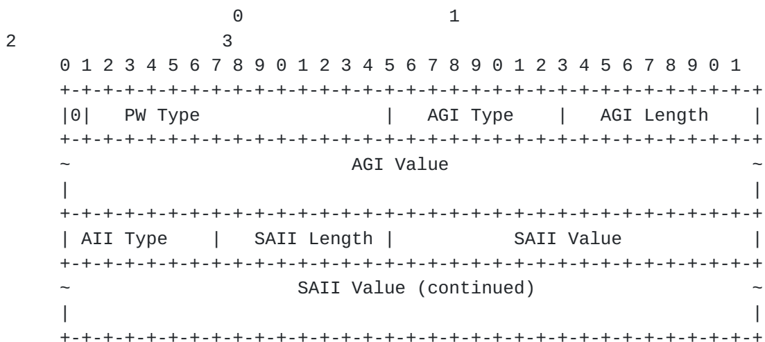
Figure 1: FEC 130 Pseudowire sub-TLV format
