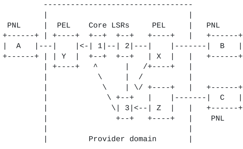
Figure 3. Unicast LSP Setup
