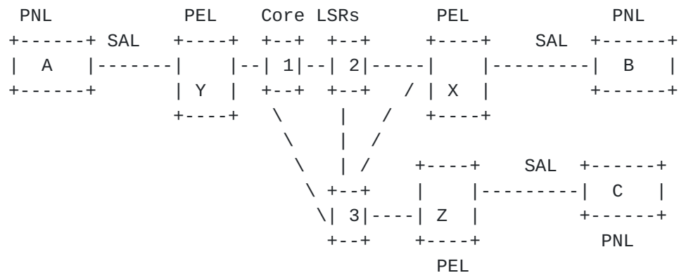
Figure 1. MPLS VPN Architecture
