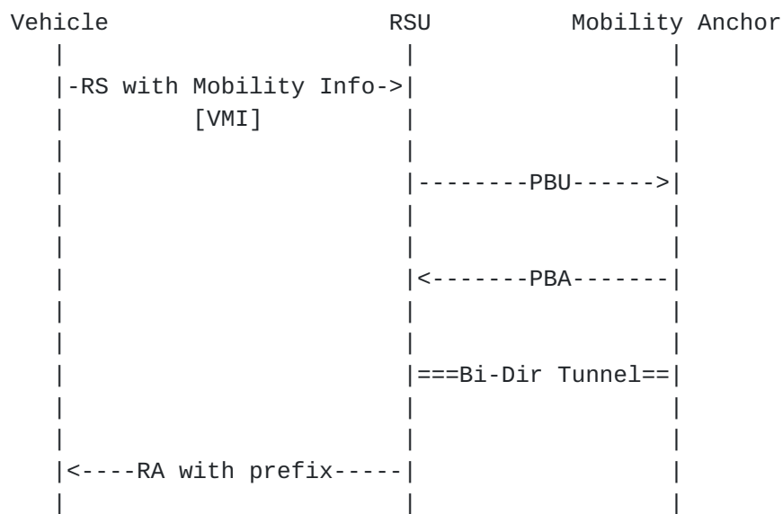
Figure 10: Message Interaction for Vehicle Attachment
