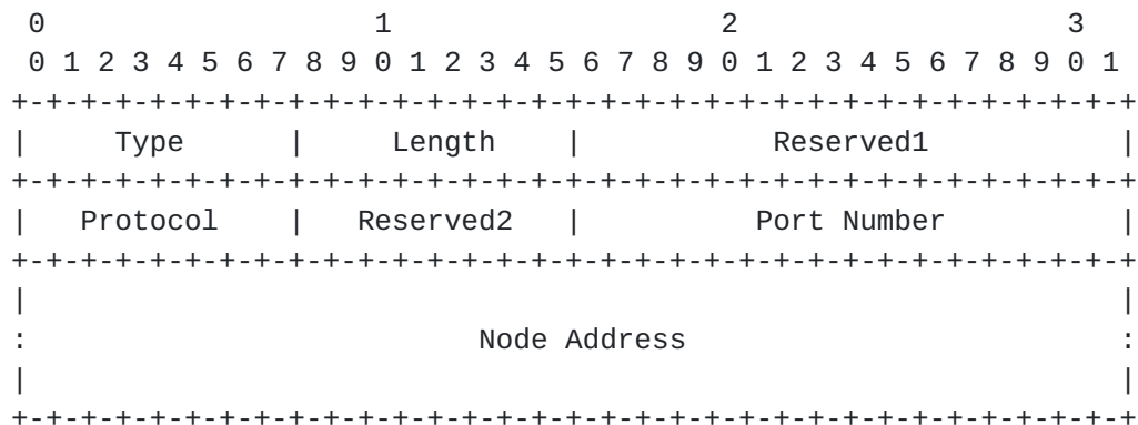
Figure 5: Vehicular Service Information (VSI) Option Format
