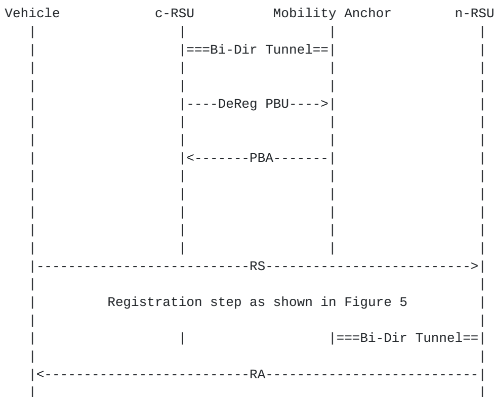
Figure 11: Message Interaction for Vehicle Handoff
