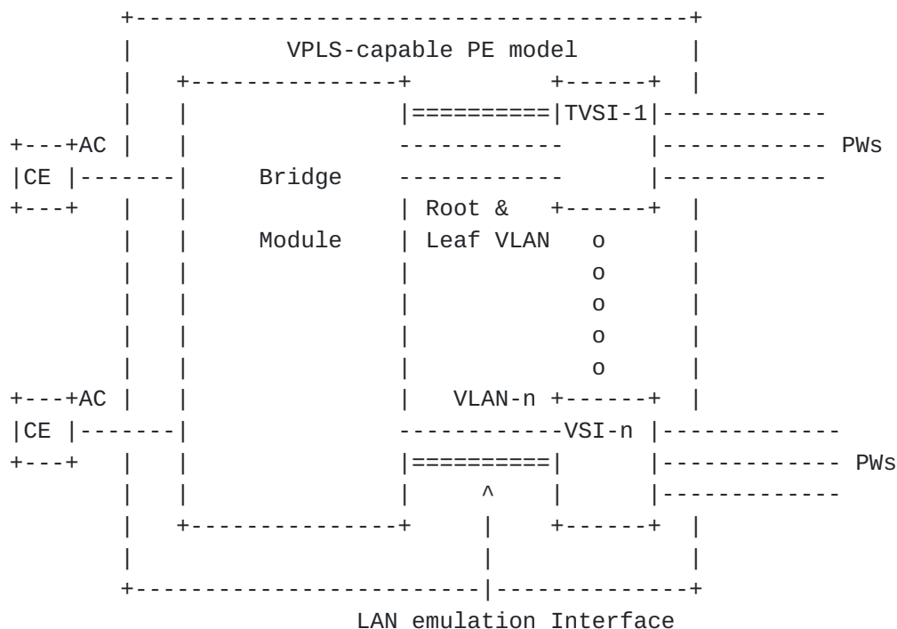
Figure 4 A VPLS PE Model for E-Tree with a Single T-VSI
