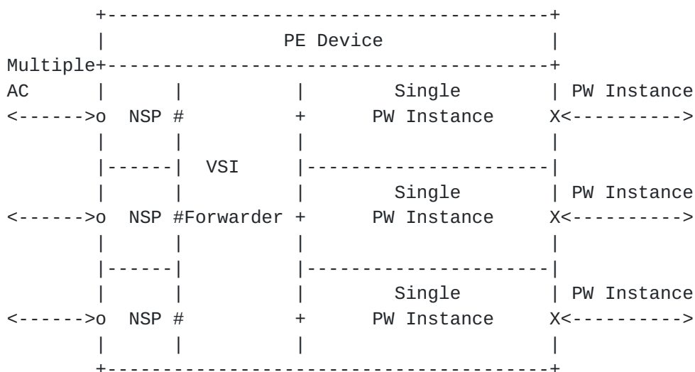
Figure A.1 A PE model with a VSI and no bridge module
