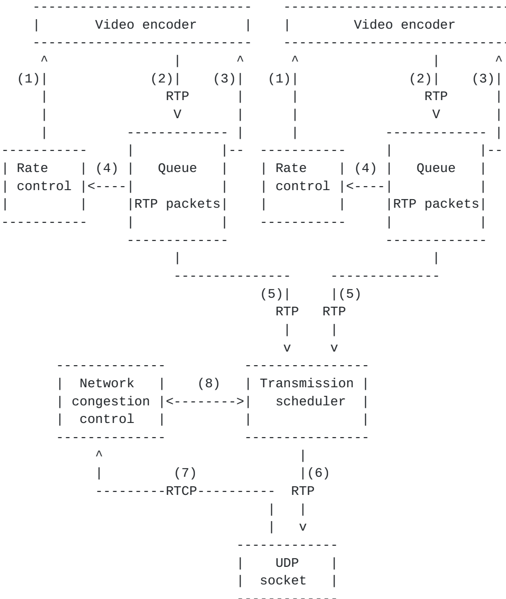
Figure 1: SReAM sender functional view
