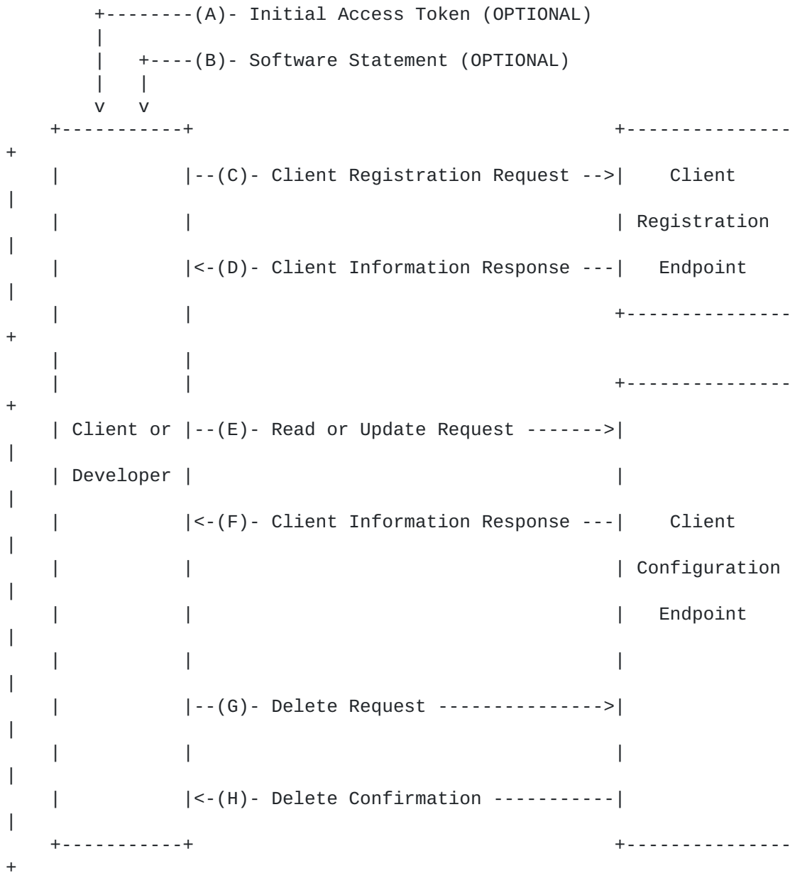
Figure 1: Abstract Extended Dynamic Client Registration Flow
