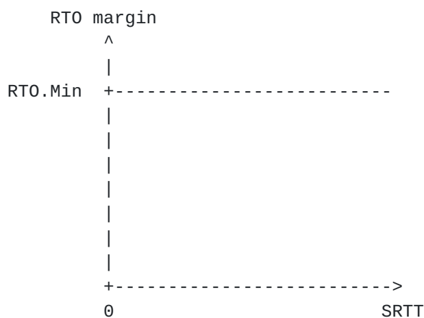
Figure 4: Relation between the RTO margin and SRTT with the new RTO calculation rules
