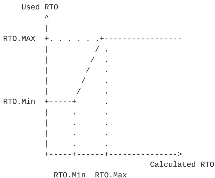
Figure 1: Relation between the calculated and used RT0 values
