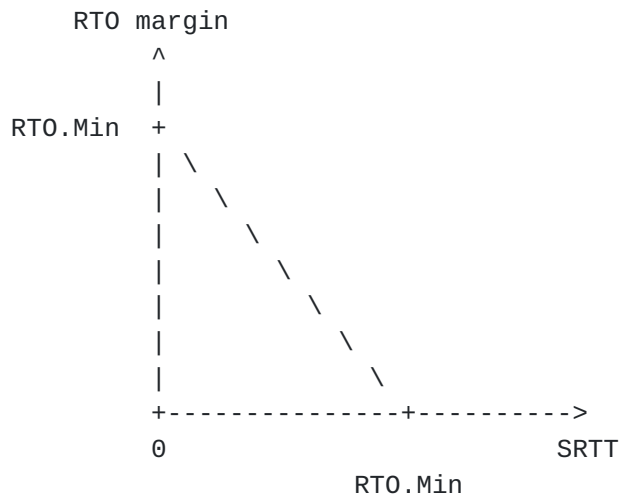
Figure 2: Relation between the RT0 margin and SRTT
