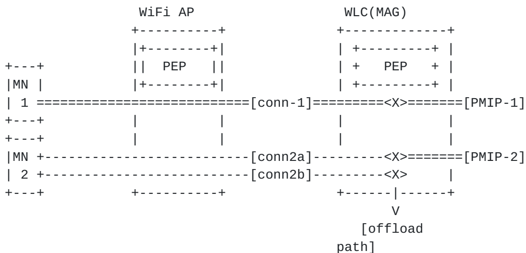
Figure 2: MN Connection and QoS Mapping
