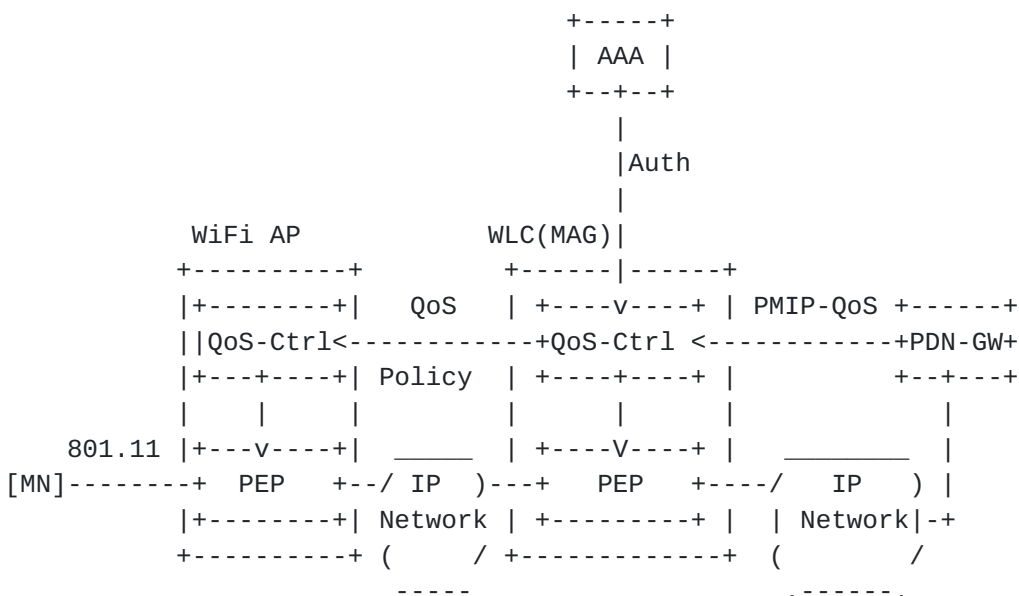
Figure 1: Architecture for provisioning QoS Policy on WiFi AP
