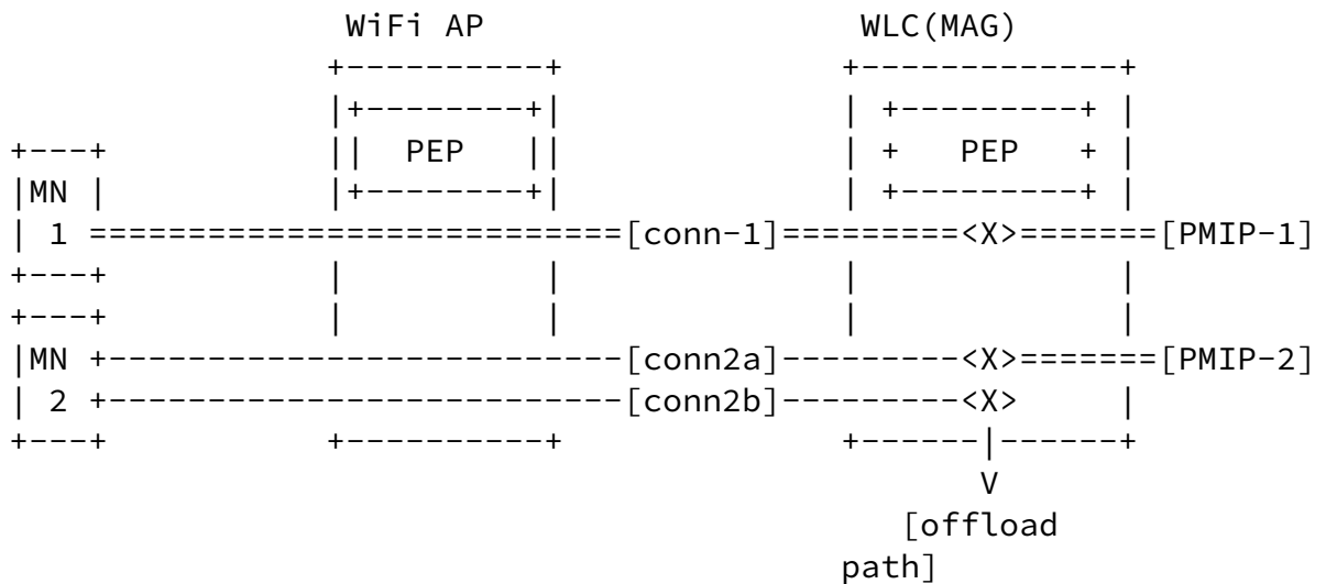
Figure 2: MN Connection and QoS Mapping
