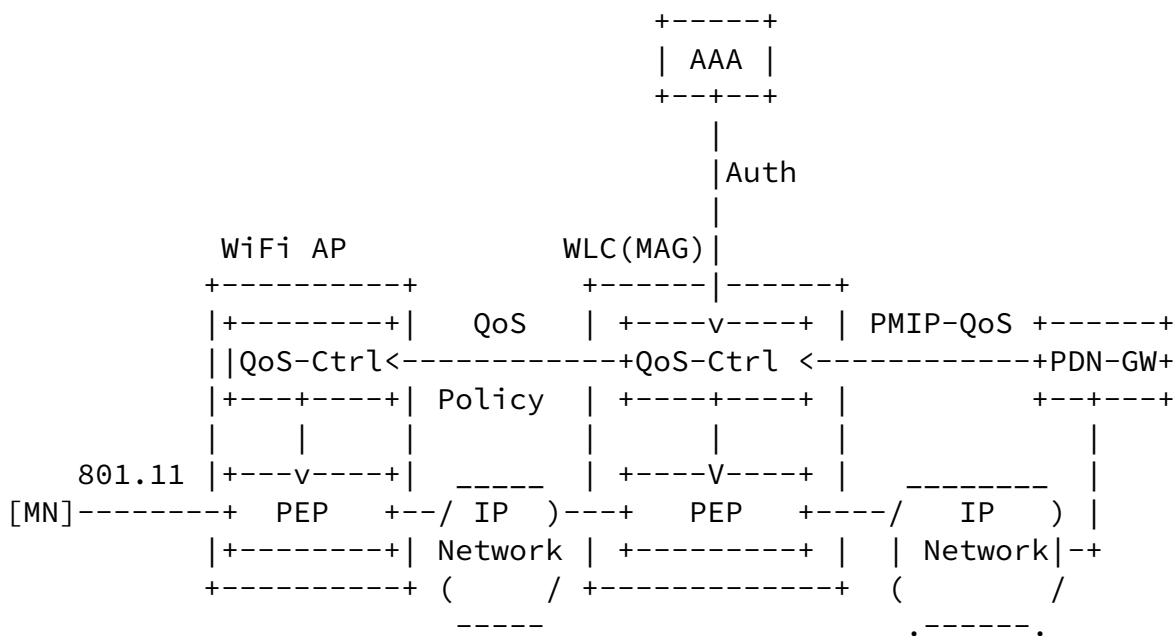
Figure 1: Architecture for provisioning QoS Policy on WiFi AP
