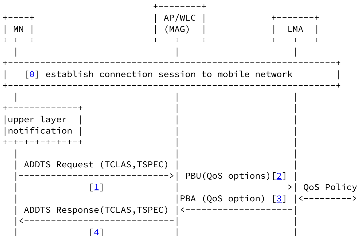
Figure 3: MN initiated QoS setup
