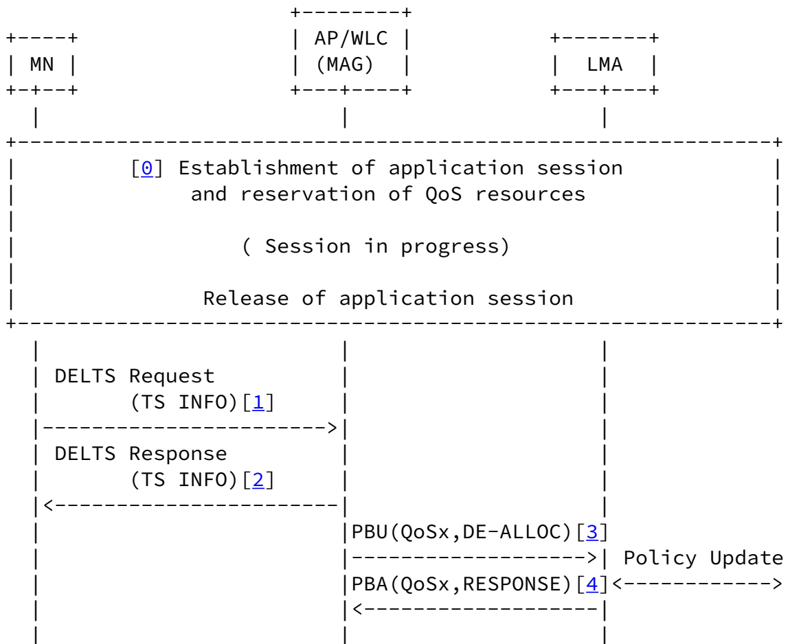
Figure 6: Network initiated QoS resource release
