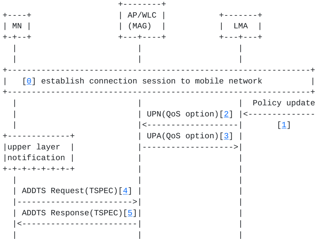
Figure 5: Network initiated QoS setup with WMM
