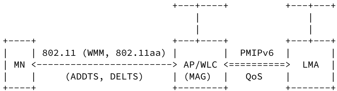
Figure 1: QoS Policy in 802.11 Access
