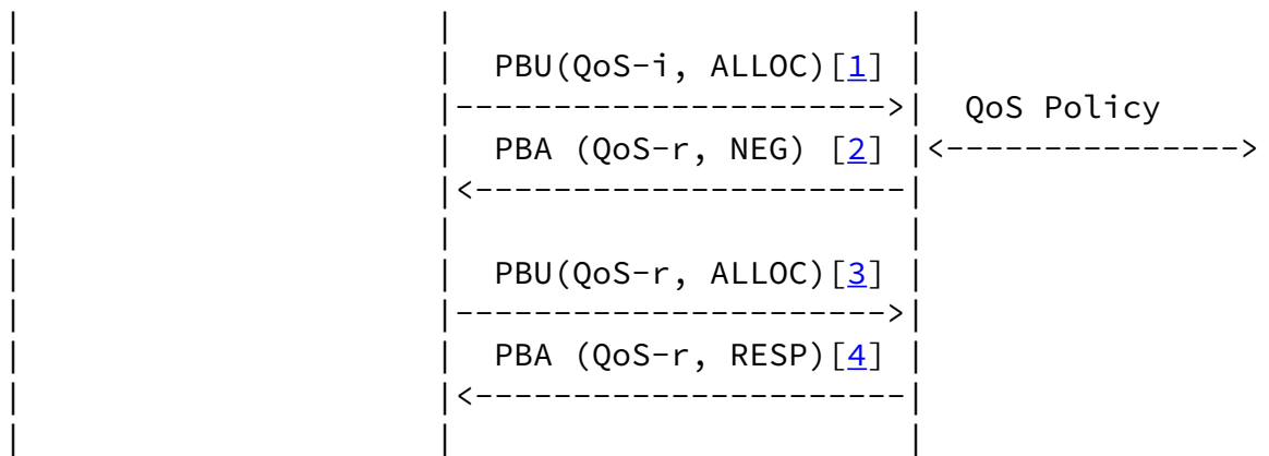
Figure 2: Default connection setup
