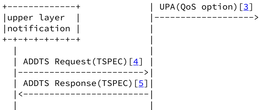
Figure 5: Network initiated QoS setup with WMM
