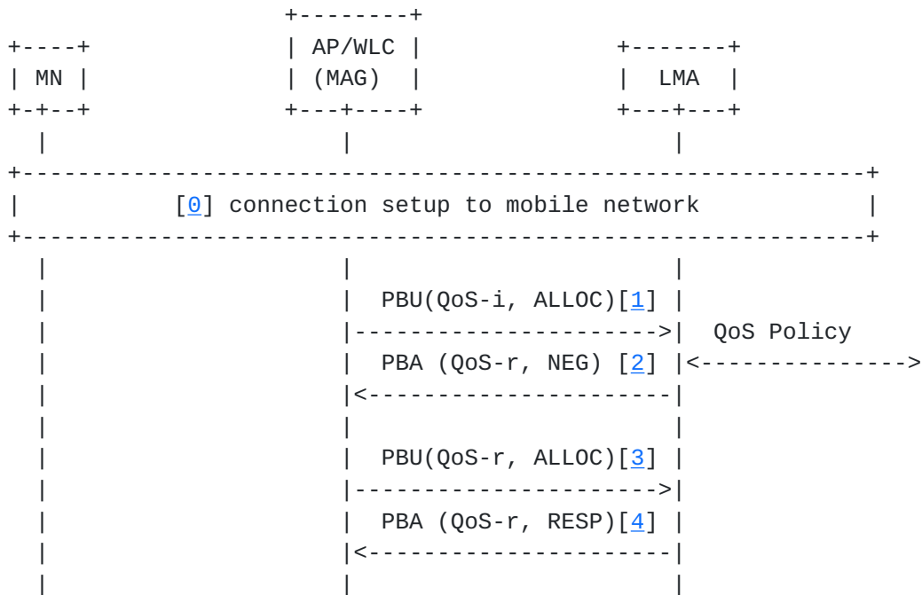
Figure 2: Default connection setup
