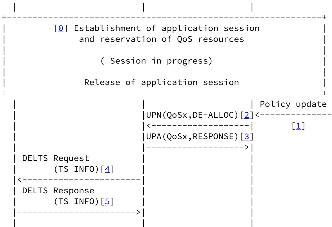
Figure 6: Network initiated QoS resource release
