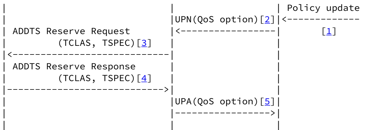
Figure 4: Network initiated QoS setup with 802.11aa
