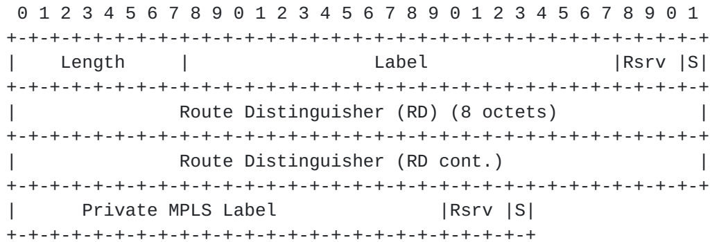
Fig 1: RFC-8277 NLRI with one Label.
