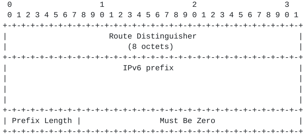
The 'Target FEC Stack' sub-TLV for IPv6 Classful Transport has a Sub-Type of [TBD], and a length of 25. The Value field consists of the RD advertised with the Classful Transport prefix, the IPv6 prefix (with trailing 0 bits to make 128 bits in all), and a prefix length, encoded as follows:
