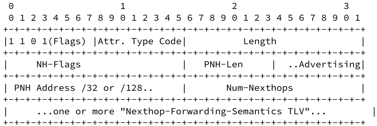
Fig 1: MultiNexthop - BGP Attribute
