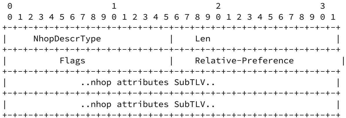
Fig 3: Nexthop Descriptor TLV
