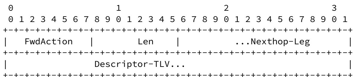
Fig 2: Nexthop Forwarding Semantics TLV
