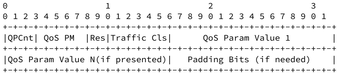
Figure 7. UQParam field
