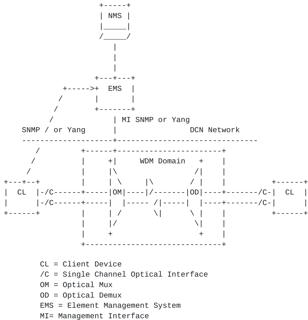
Figure 3: Connecting Single Channel optical interfaces to the Transport Management system
