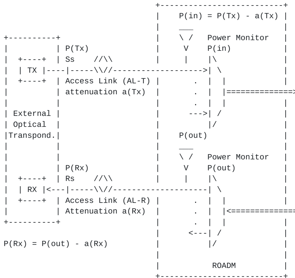
Figure 5 Access Link Power Monitoring
