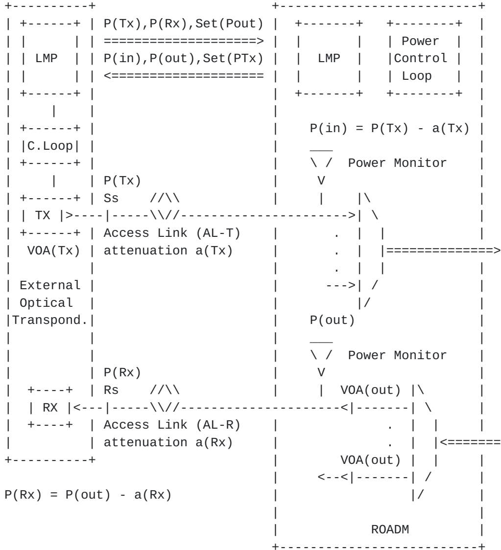
Figure 7: Extended LMP Model
