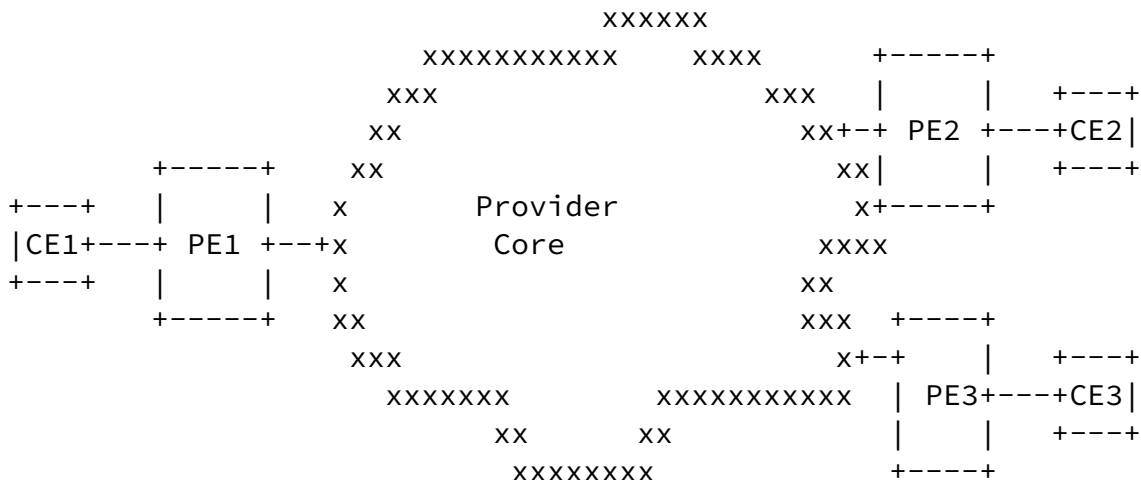
MVPN topology
